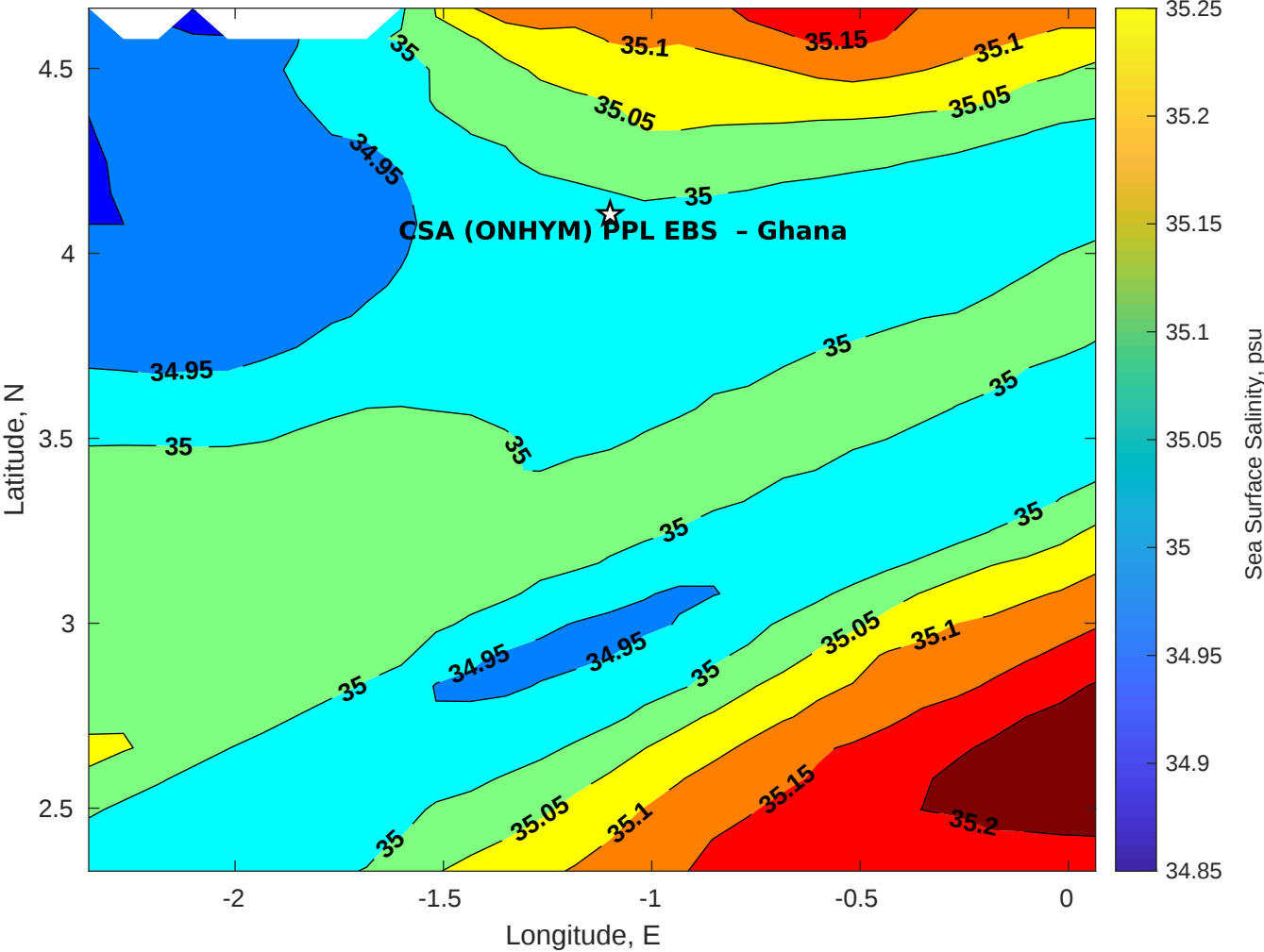
Surface Salinity for CSA (ONHYM) PPL EBS - Ghana at 10-Jul-2025 00:00:00
