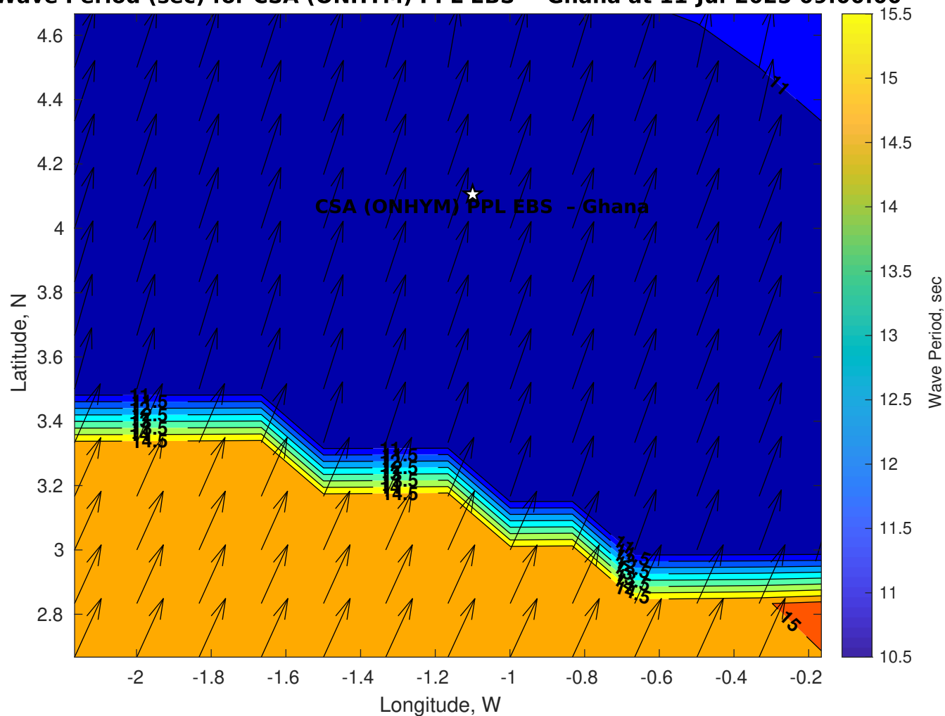
Wave Period (sec) for CSA (ONHYM) PPL EBS - Ghana at 11-Jul-2025 09:00:00
