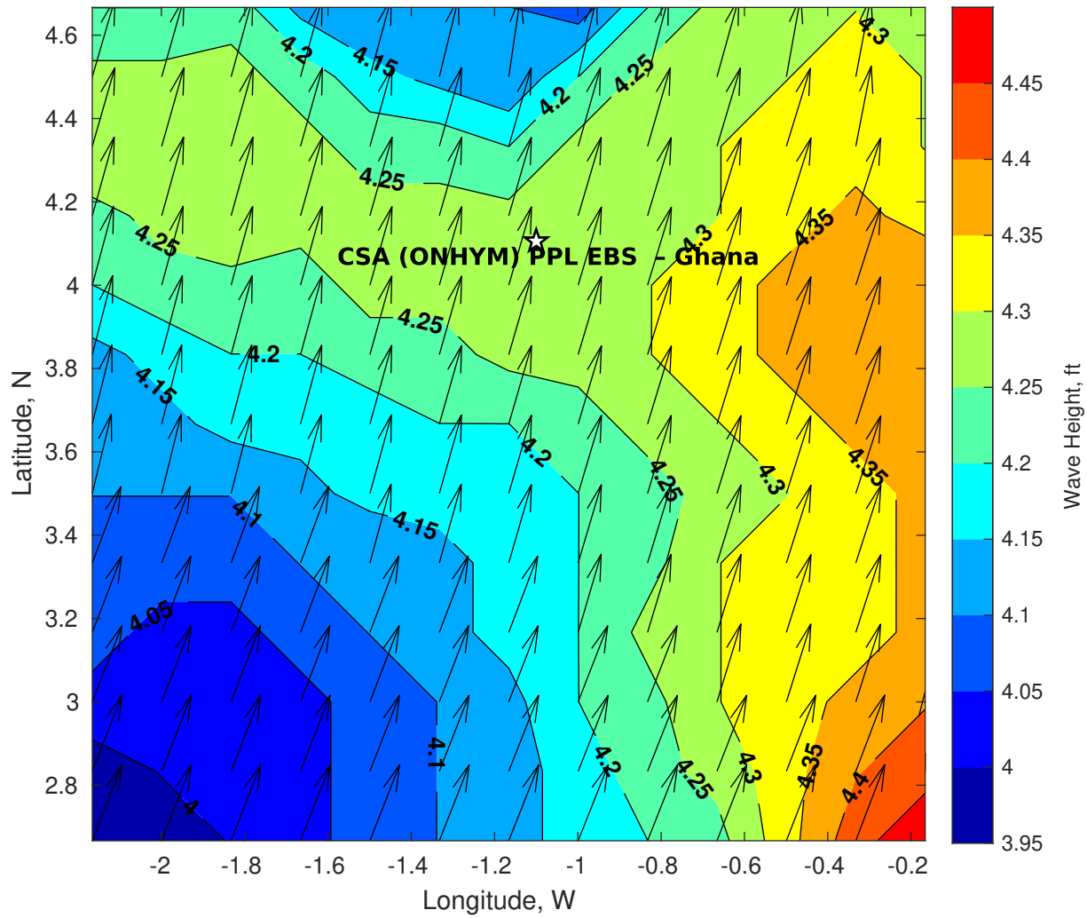
Wave Height (ft) for CSA (ONHYM) PPL EBS - Ghana at 11-Jul-2025 09:00:00
