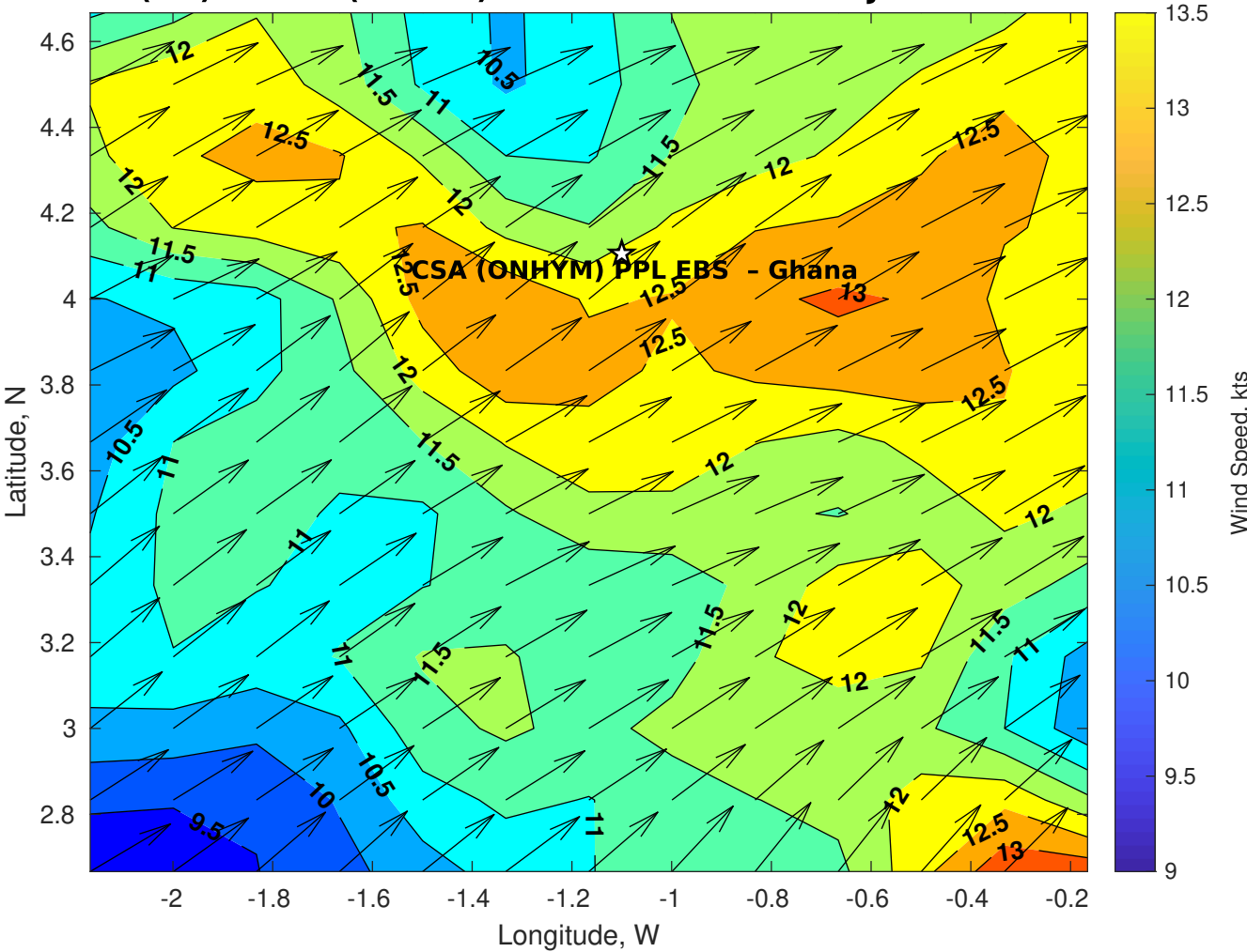
Winds (kts) for CSA (ONHYM) PPL EBS - Ghana at 11-Jul-2025 09:00:00
