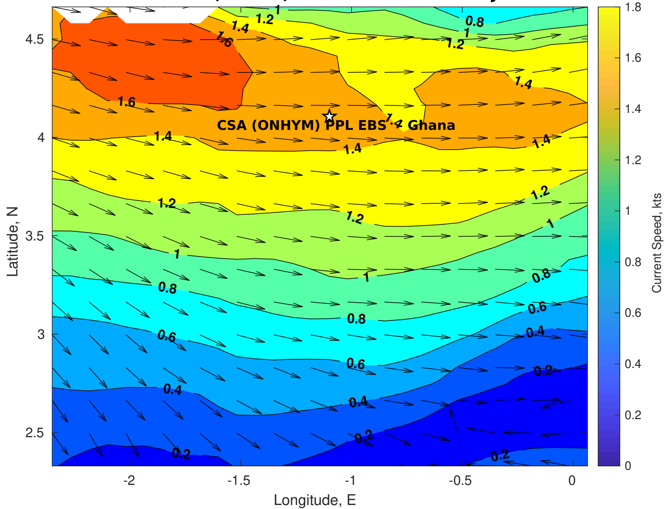
Surface Currents for CSA (ONHYM) PPL EBS - Ghana at 10-Jul-2025 00:00:00
