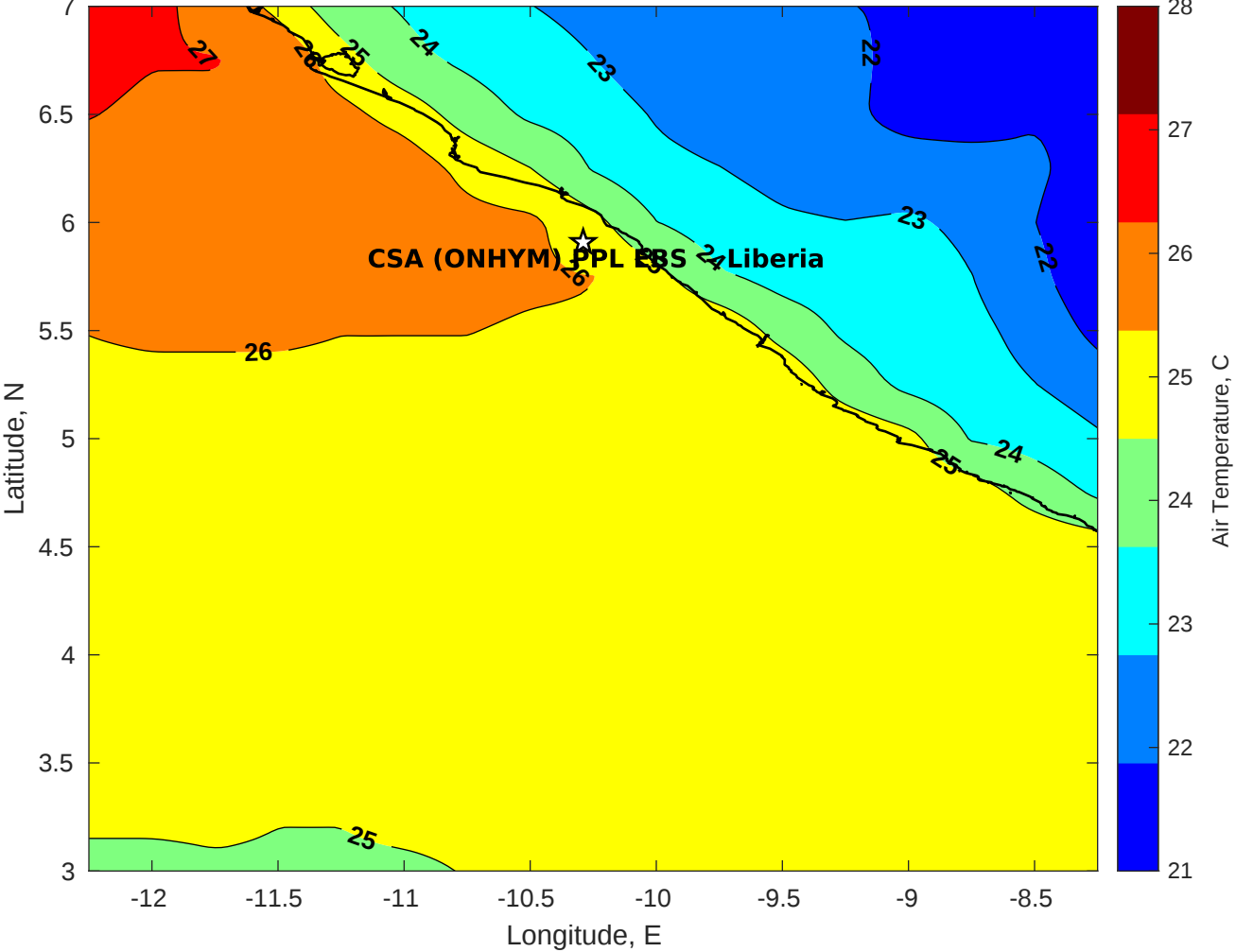
Air Temperature (C) for CSA (ONHYM) PPL EBS - Liberia at 11-Jul-2025
