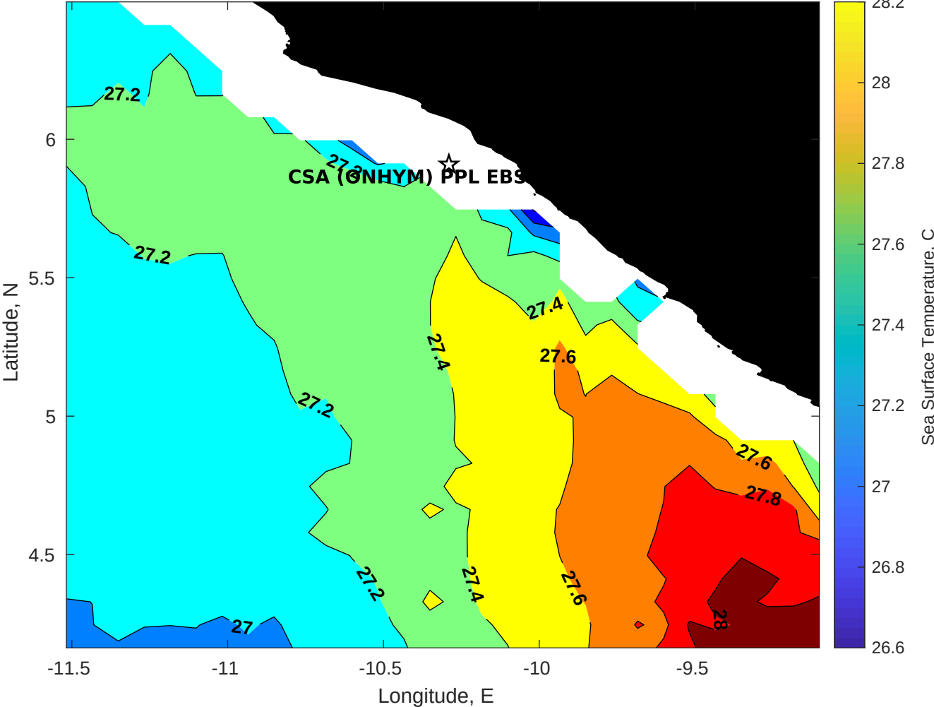
SST for CSA (ONHYM) PPL EBS - Liberia at 10-Jul-2025 00:00:00
