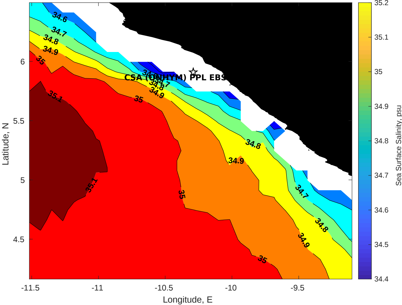
Surface Salinity for CSA (ONHYM) PPL EBS - Liberia at 10-Jul-2025 00:00:00
