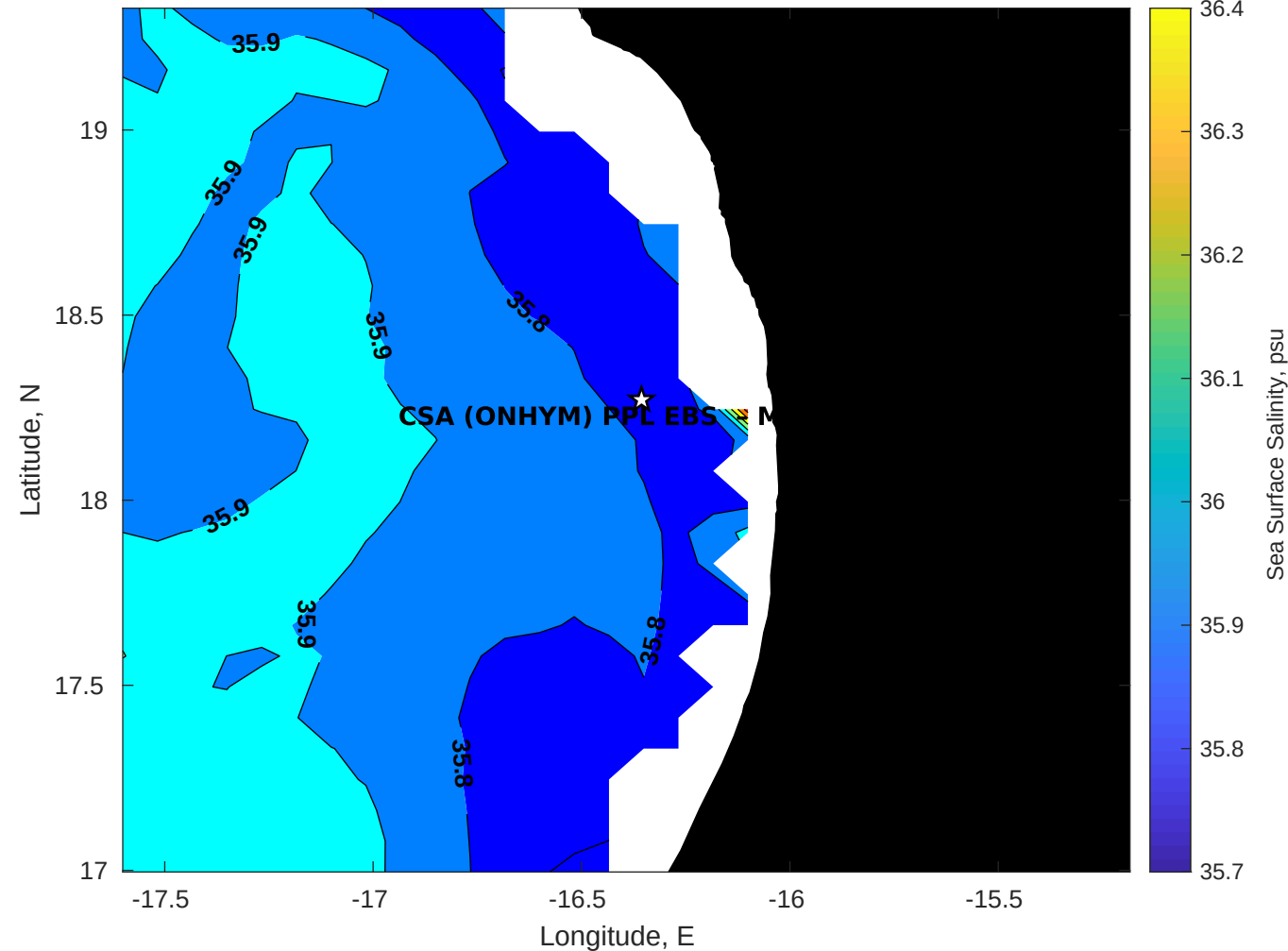
Surface Salinity for CSA (ONHYM) PPL EBS - Mauritania at 10-Jul-2025 00:00:00
