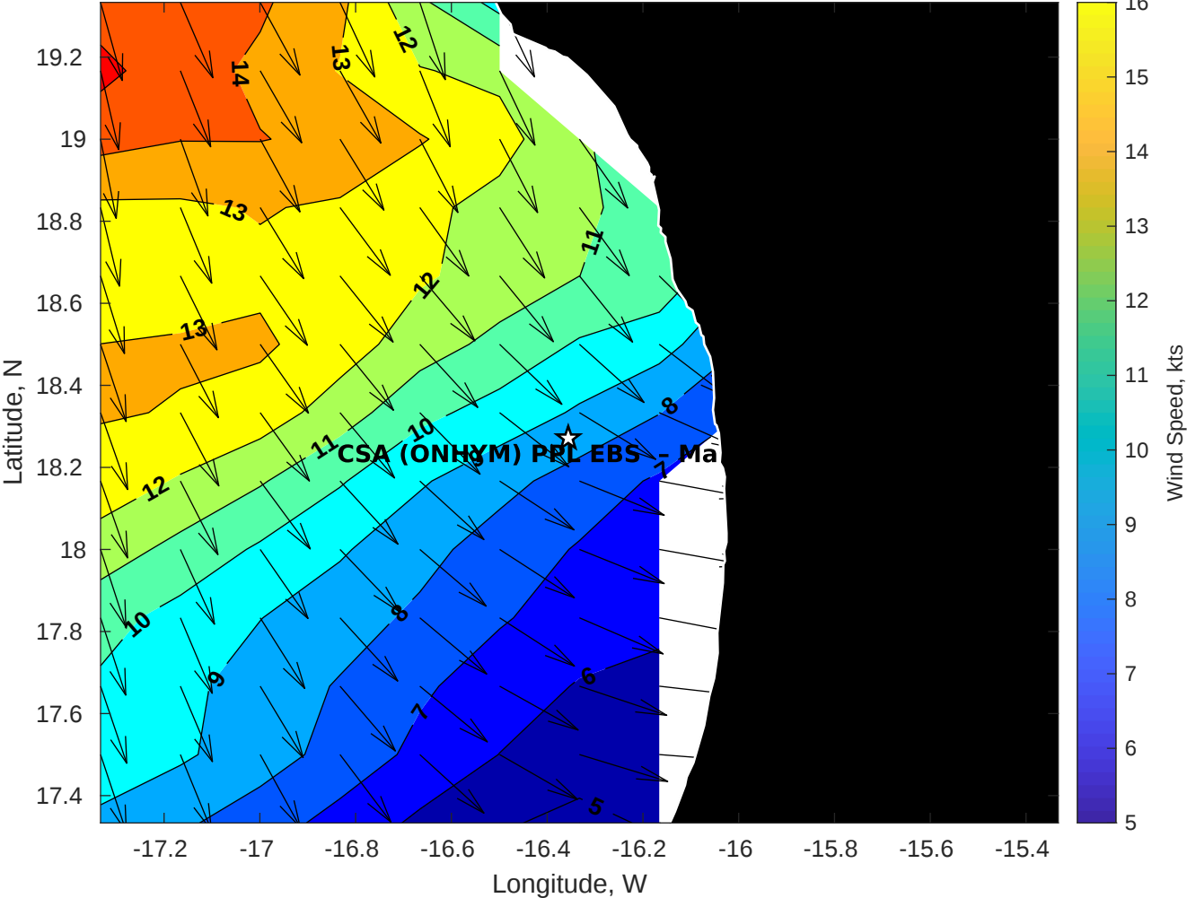
Winds (kts) for CSA (ONHYM) PPL EBS - Mauritania at 11-Jul-2025 09:00:00
