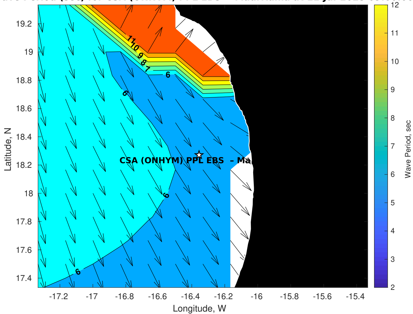
Wave Period (sec) for CSA (ONHYM) PPL EBS - Mauritania at 11-Jul-2025 09:00:00
