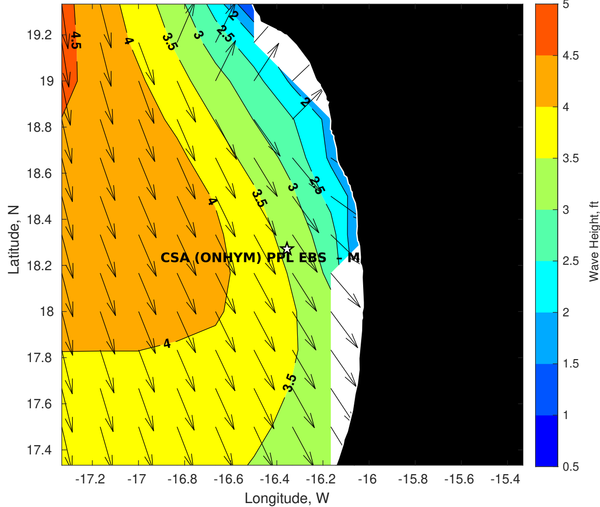
Wave Height (ft) for CSA (ONHYM) PPL EBS - Mauritania at 11-Jul-2025 09:00:00
