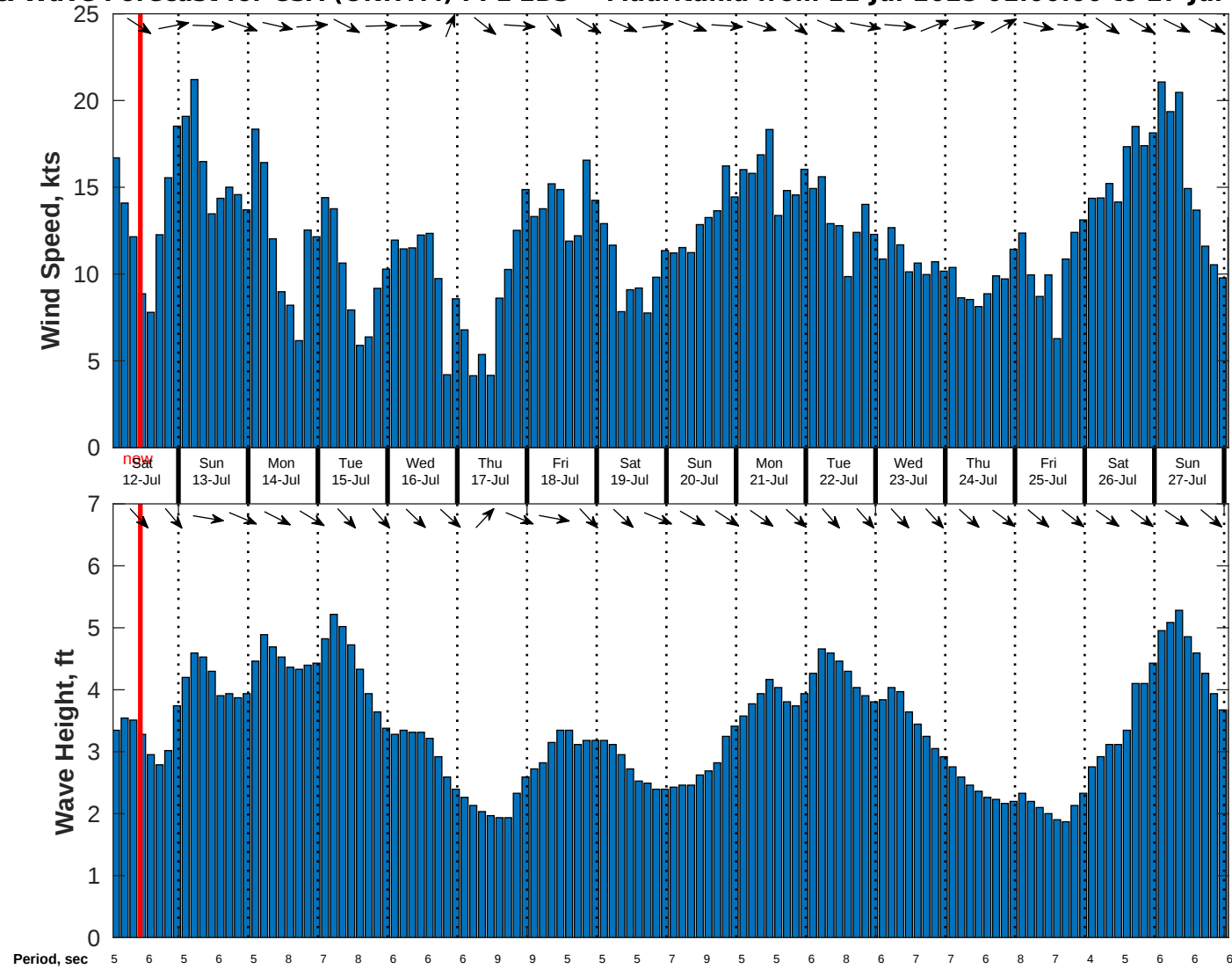
Wind & Wave Forecast for CSA (ONHYM) PPL EBS - Mauritania from 11-Jul-2025 01:00:00 to 27-Jul-2025 01:00:00
