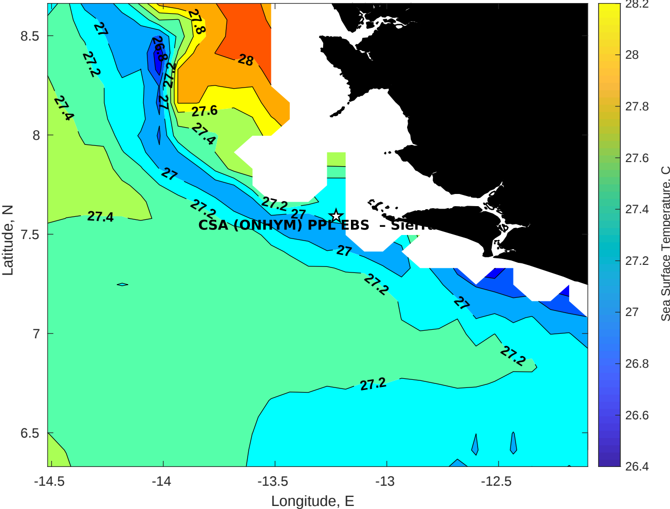
SST for CSA (ONHYM) PPL EBS - Sierra Leone at 10-Jul-2025 00:00:00
