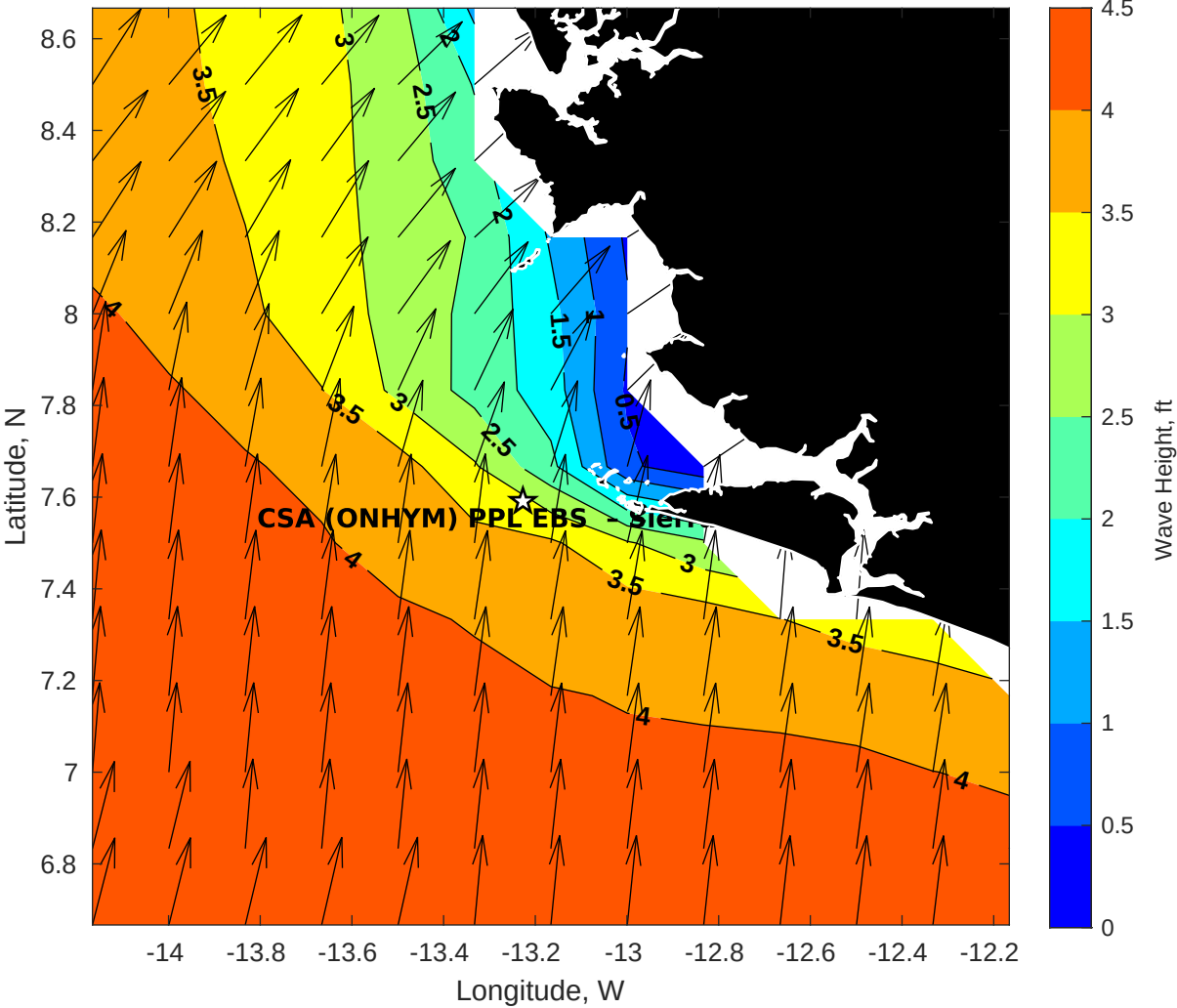
Wave Height (ft) for CSA (ONHYM) PPL EBS - Sierra Leone at 11-Jul-2025 09:00:00
