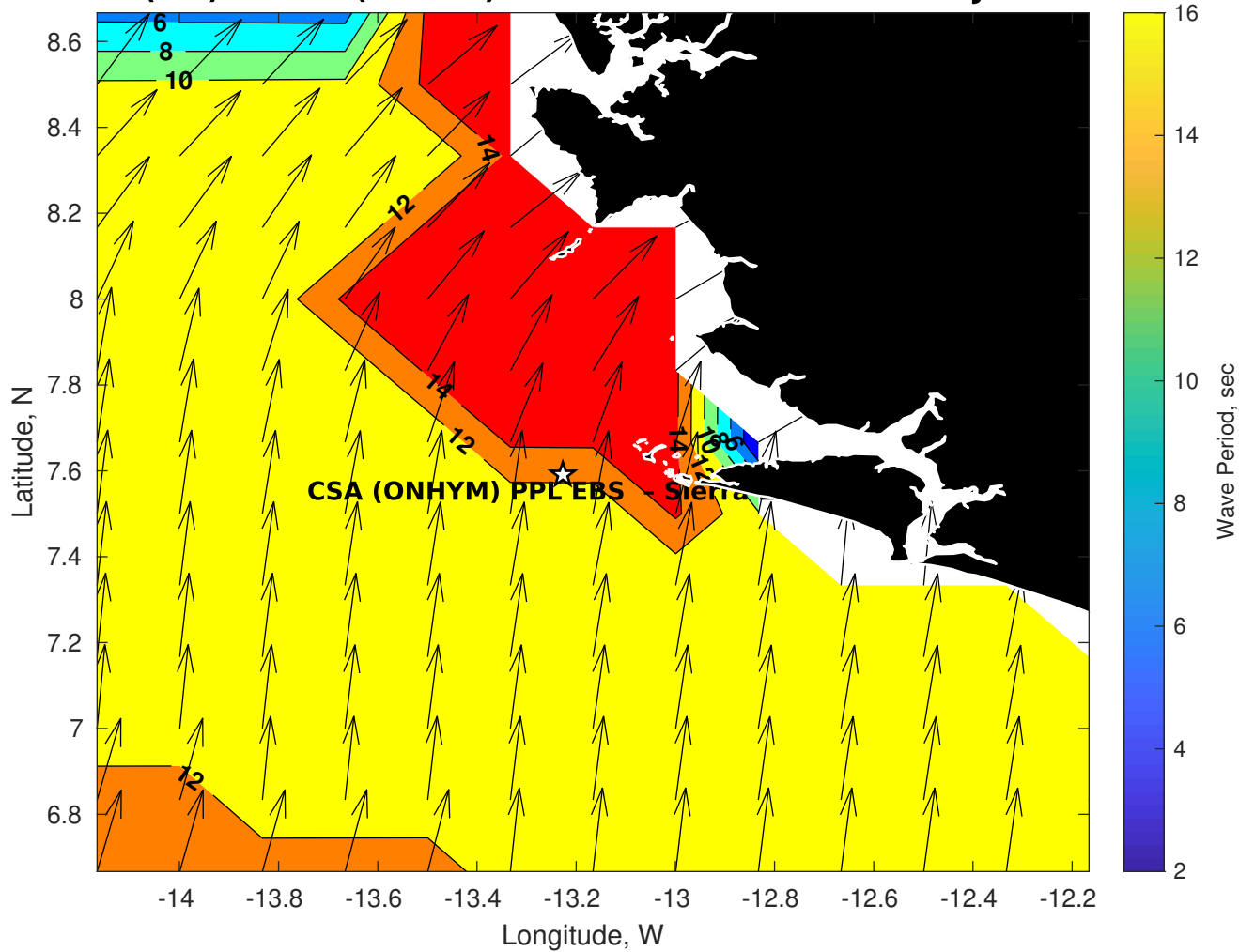
Wave Period (sec) for CSA (ONHYM) PPL EBS - Sierra Leone at 11-Jul-2025 09:00:00
