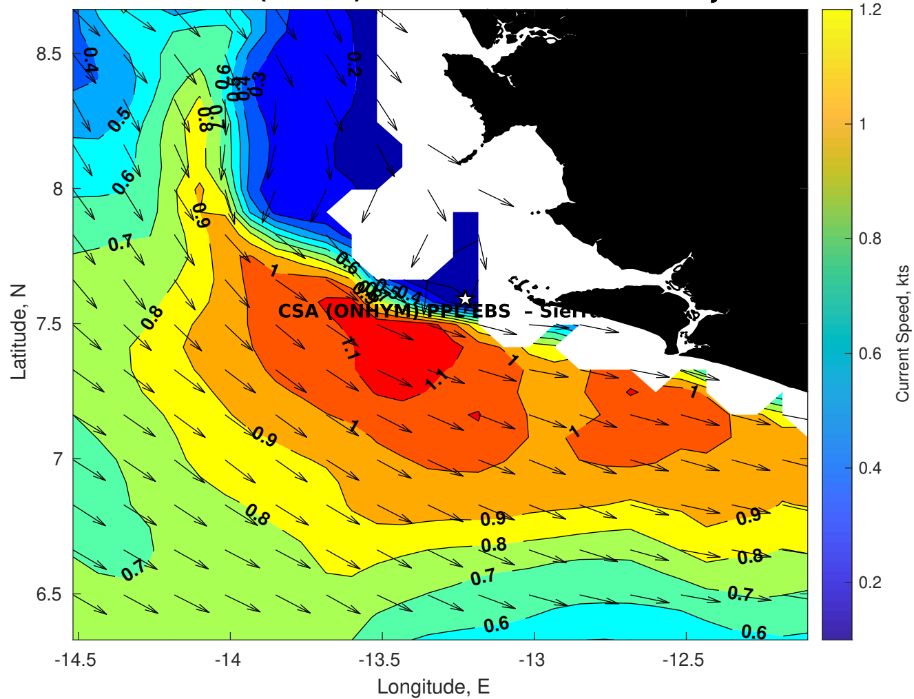
Surface Currents for CSA (ONHYM) PPL EBS - Sierra Leone at 10-Jul-2025 00:00:00
