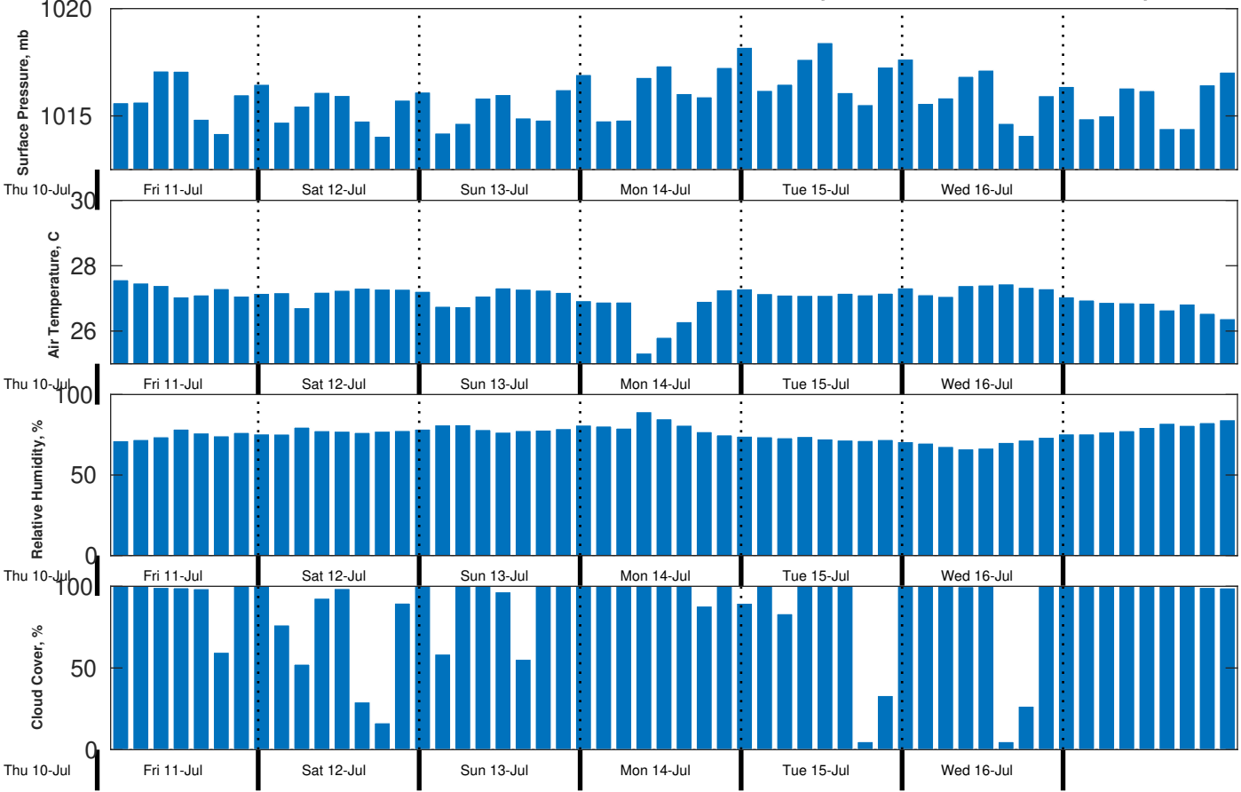
Met Forecast for CSA (ONHYM) PPL EBS - Sierra Leone from 11-Jul-2025 00:00:00 to 18-Jul-2025 00:00:00
