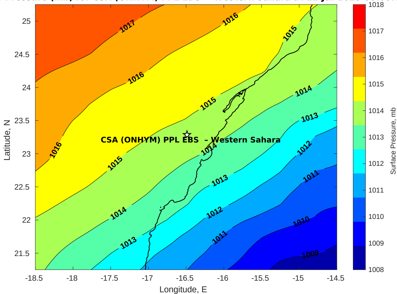
Surface Pressure (mb) for CSA (ONHYM) PPL EBS - Western Sahara at 12-Jul-2025 00:00:00
