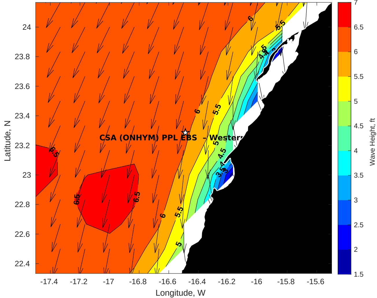
Wave Height (ft) for CSA (ONHYM) PPL EBS - Western Sahara at 11-Jul-2025 09:00:00
