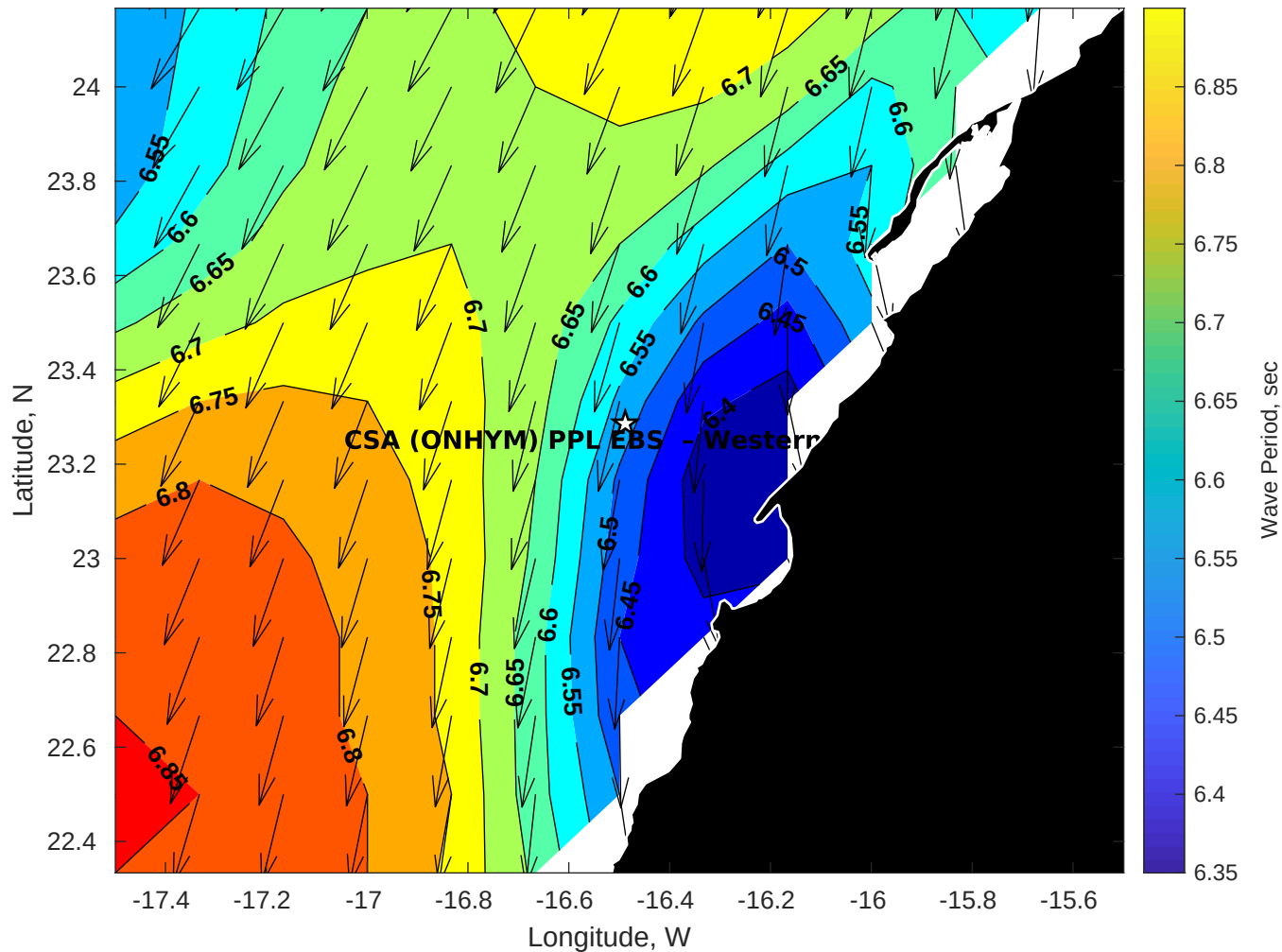
Wave Period (sec) for CSA (ONHYM) PPL EBS - Western Sahara at 11-Jul-2025 09:00:00
