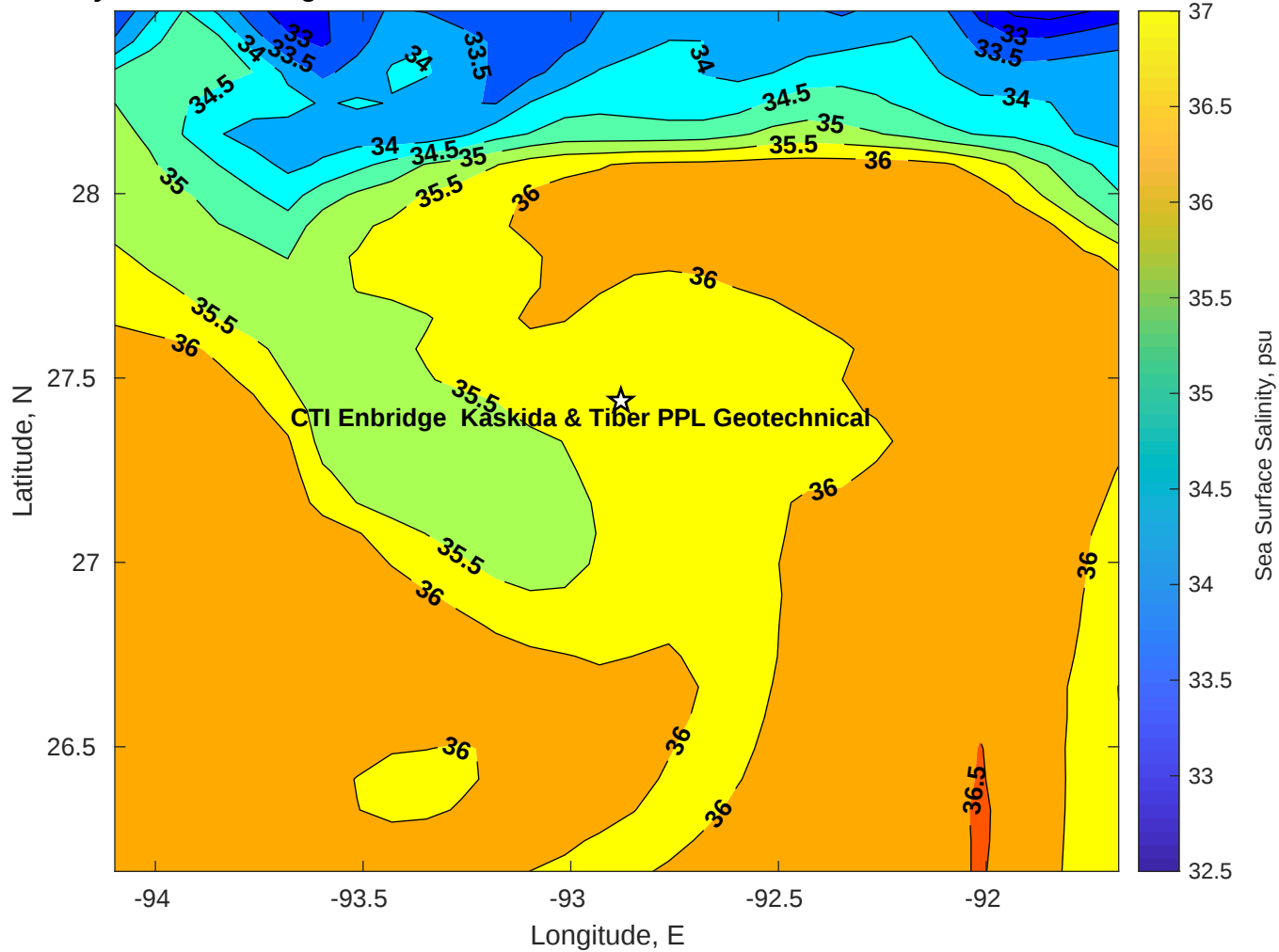
Surface Salinity for CTI Enbridge Kaskida & Tiber PPL Geotechnical at 10-Jul-2025 00:00:00
