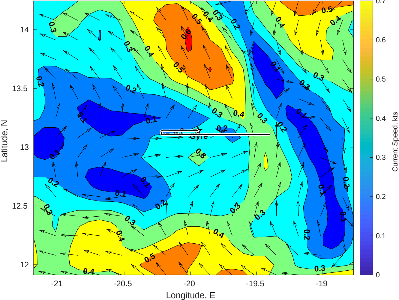
Surface Currents for Gyre at 10-Jul-2025 00:00:00
