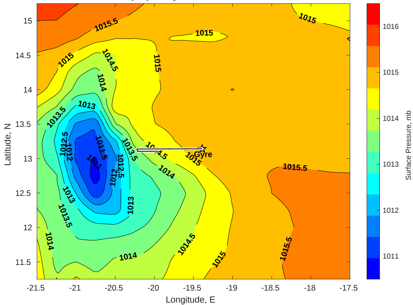
Surface Pressure (mb) for Gyre at 12-Jul-2025 00:00:00
