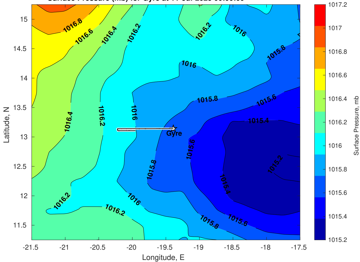
Surface Pressure (mb) for Gyre at 11-Jul-2025 00:00:00
