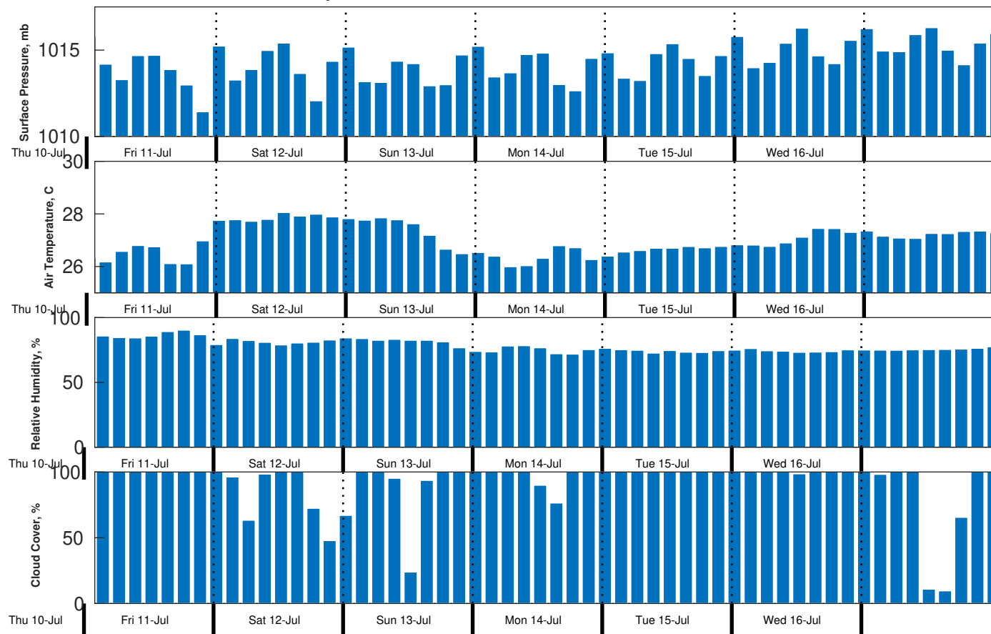
Met Forecast for Gyre from 10-Jul-2025 23:00:00 to 17-Jul-2025 23:00:00
