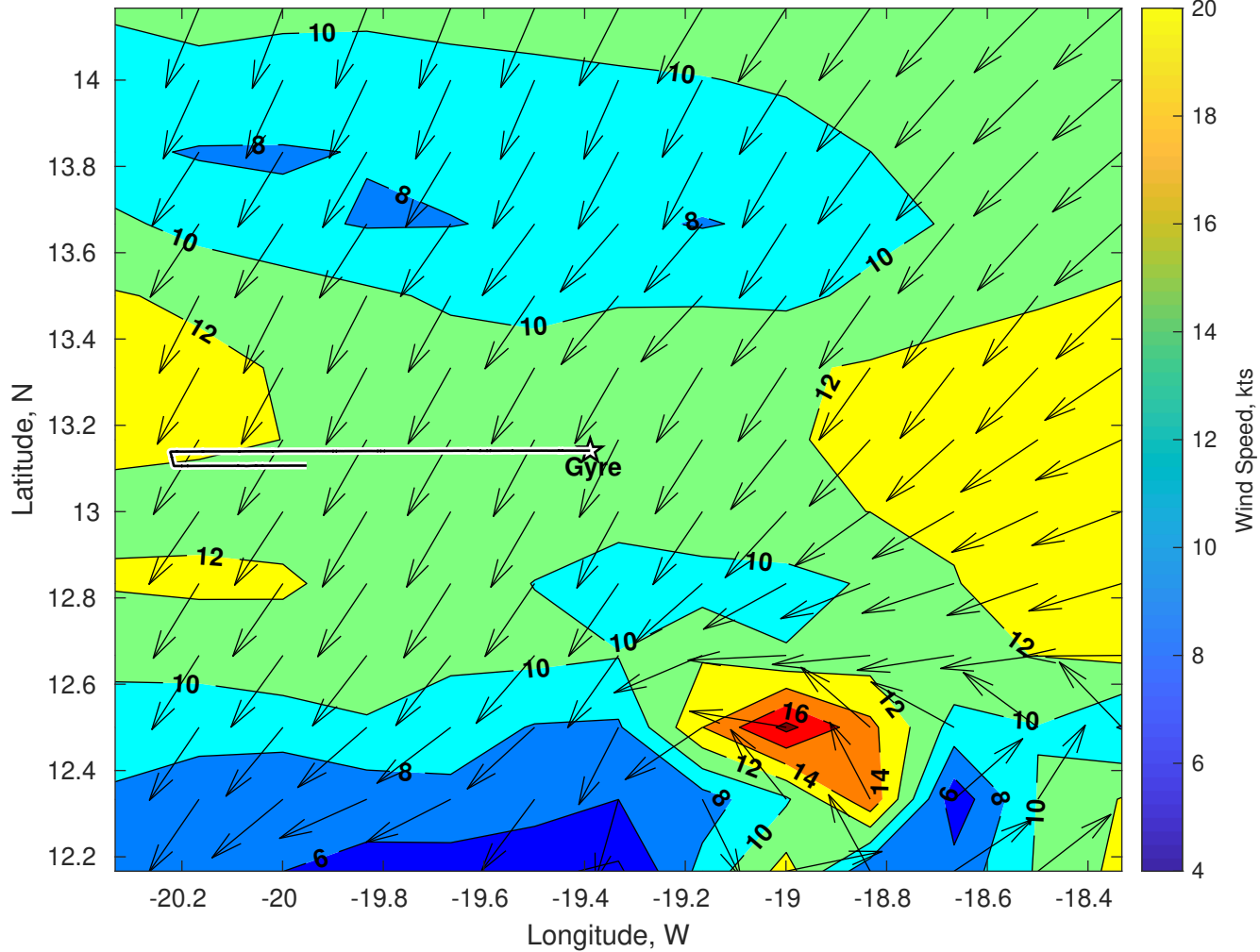
Winds (kts) for Gyre at 11-Jul-2025 09:00:00
