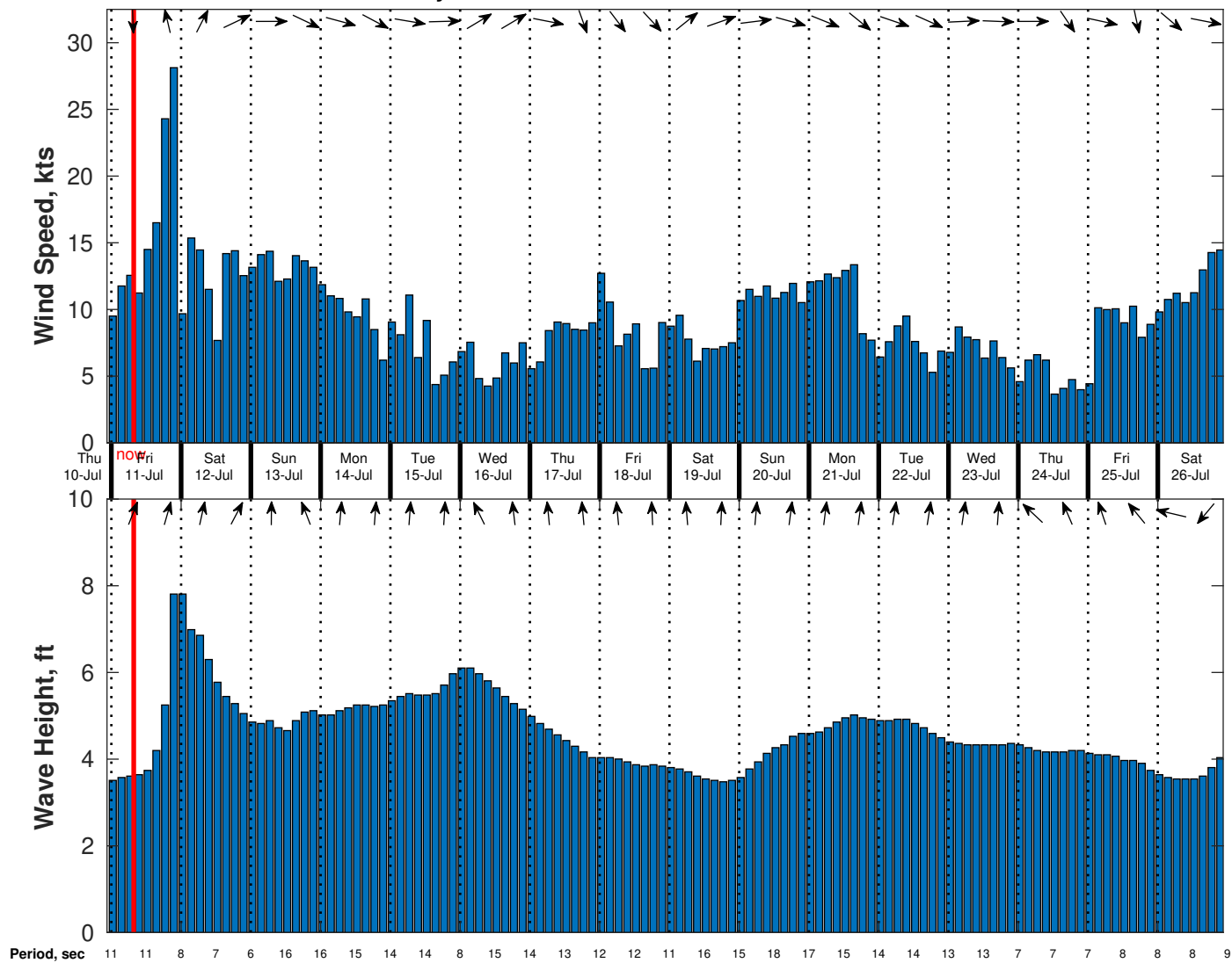
Wind & Wave Forecast for Gyre from 10-Jul-2025 23:00:00 to 26-Jul-2025 23:00:00
