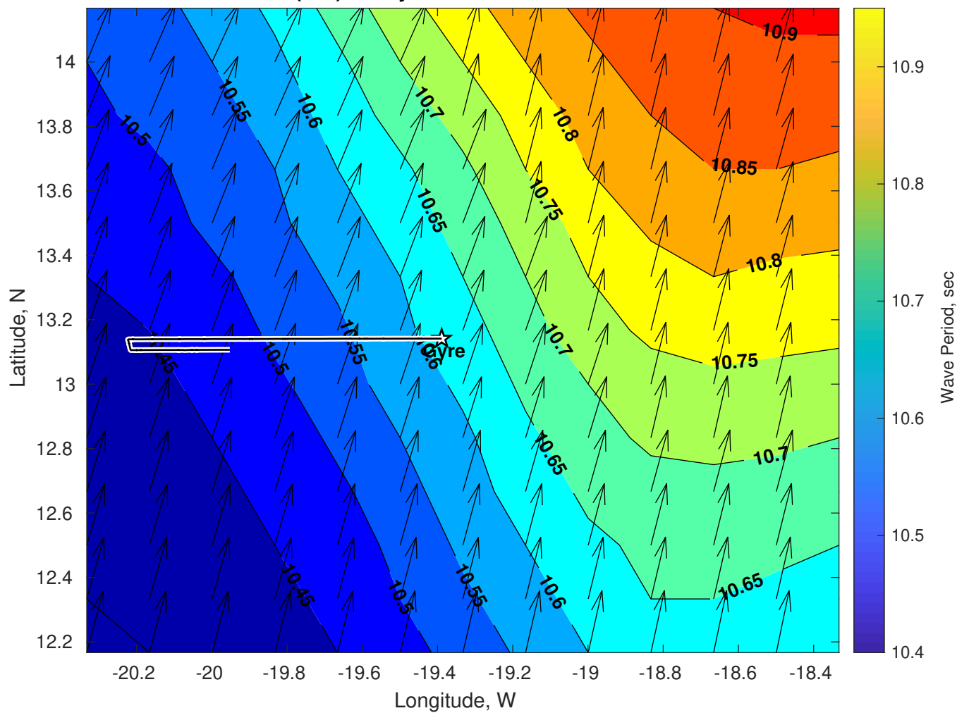
Wave Period (sec) for Gyre at 11-Jul-2025 09:00:00
