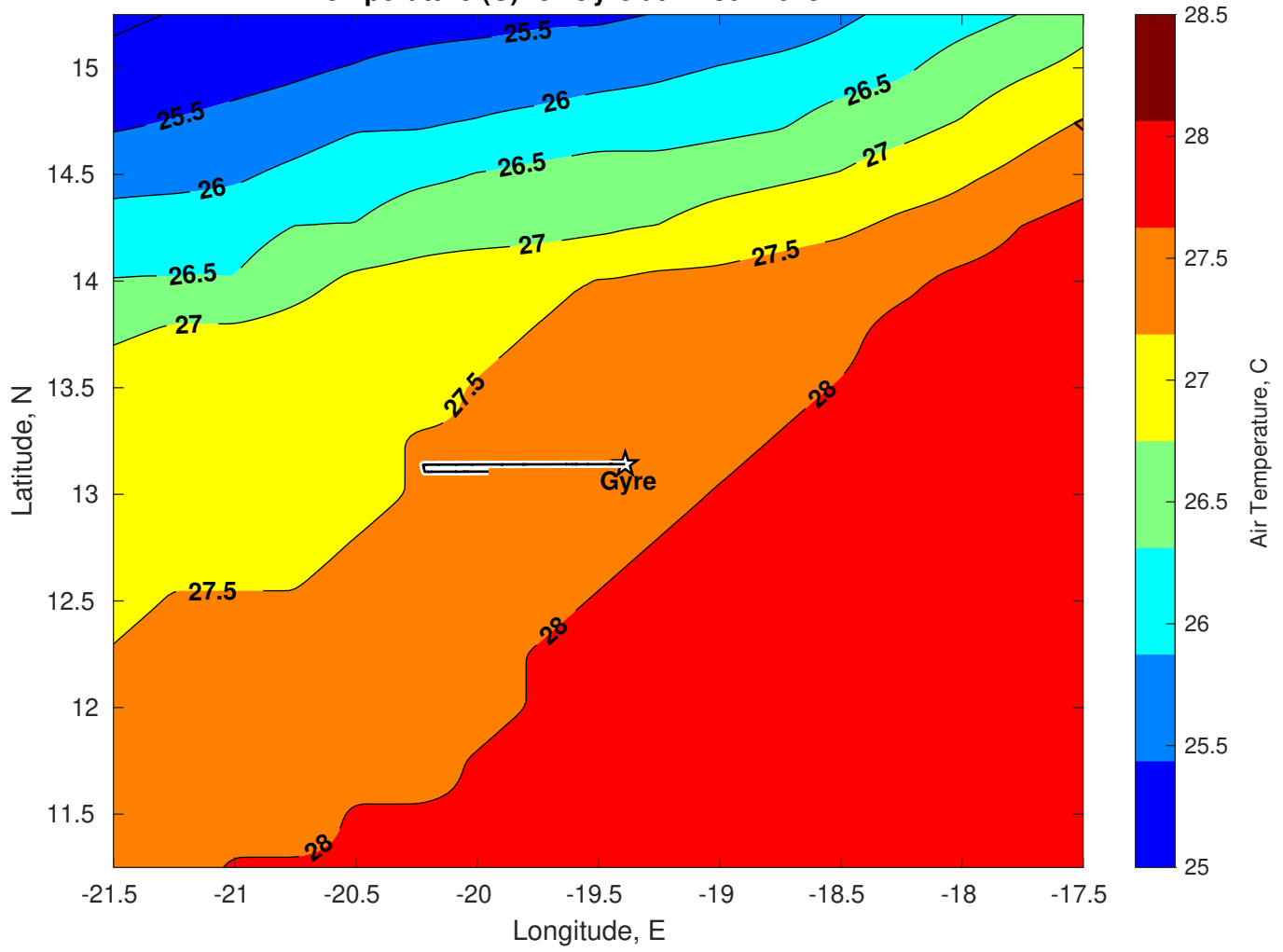
Air Temperature (C) for Gyre at 11-Jul-2025
