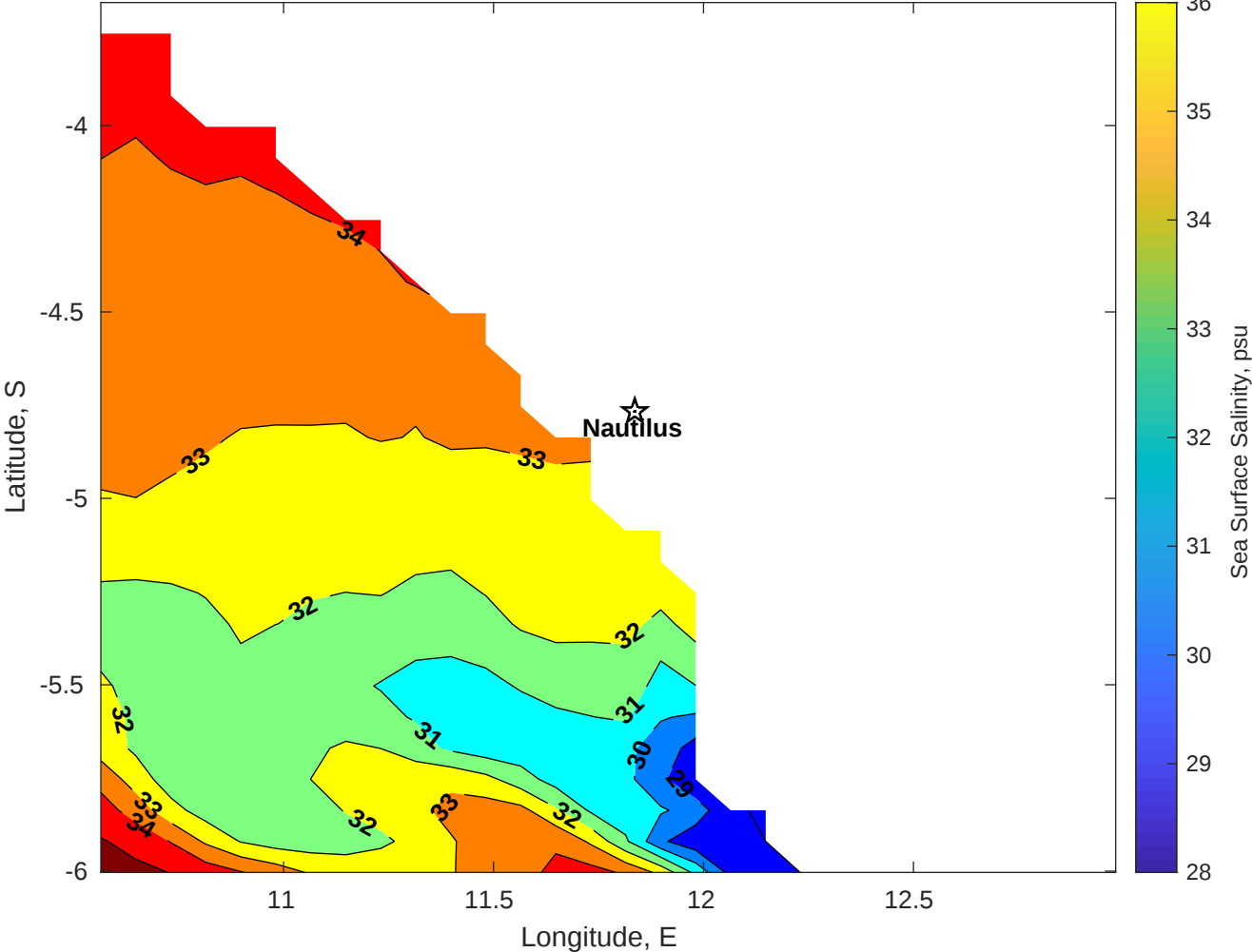
Surface Salinity for Nautilus at 10-Jul-2025 00:00:00
