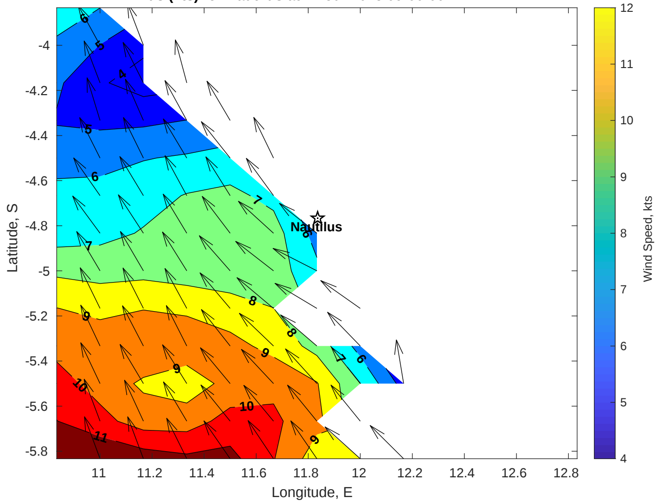
Winds (kts) for Nautilus at 11-Jul-2025 09:00:00
