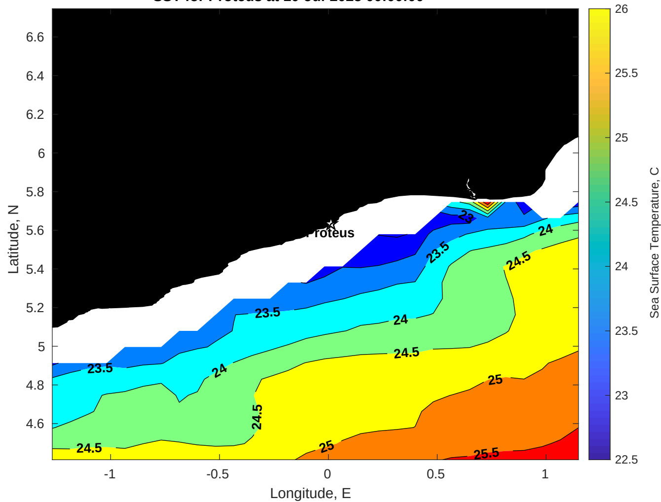
SST for Proteus at 10-Jul-2025 00:00:00
