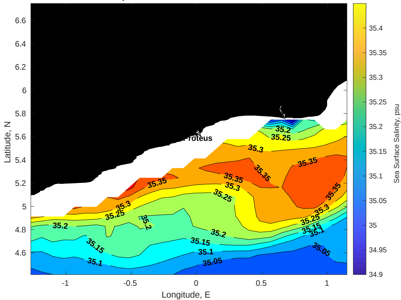
Surface Salinity for Proteus at 10-Jul-2025 00:00:00
