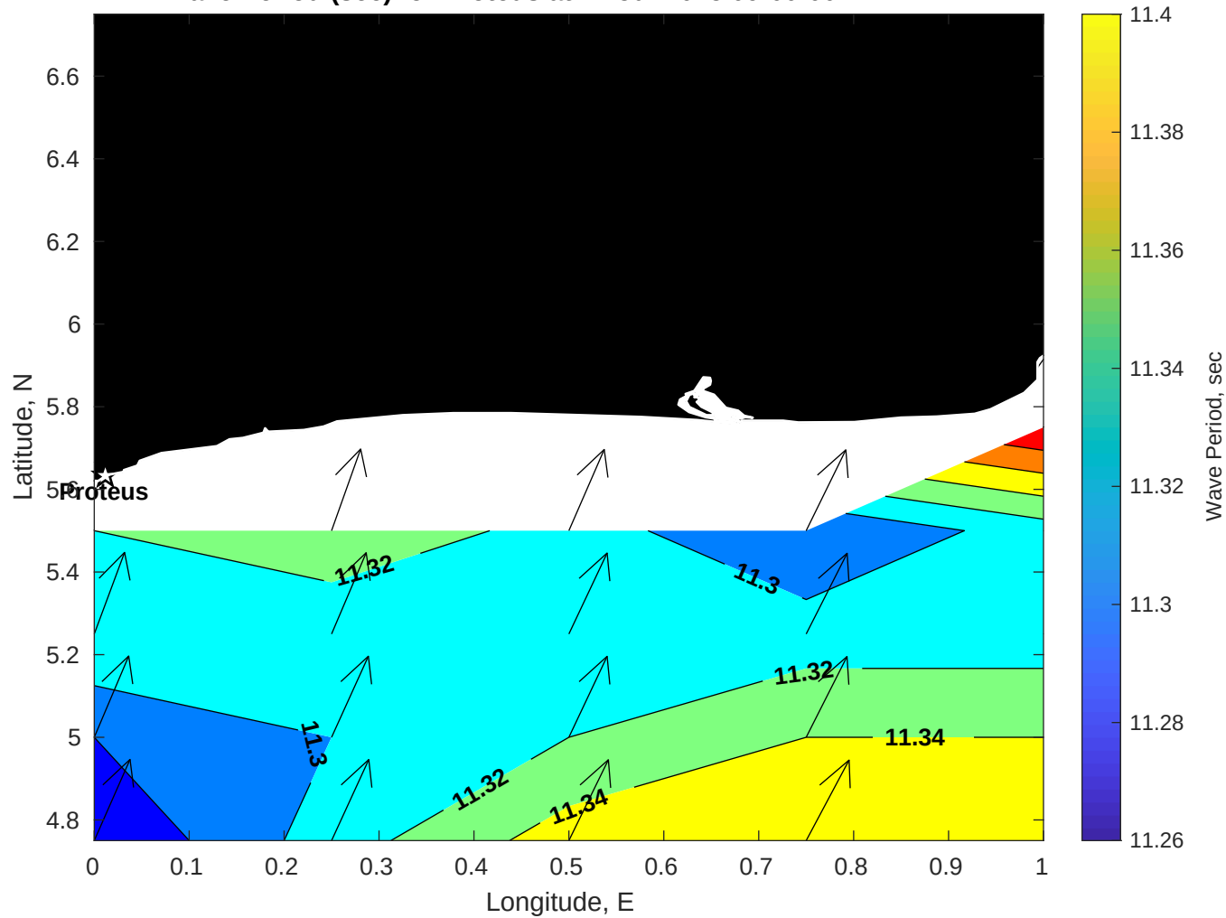
Wave Period (sec) for Proteus at 11-Jul-2025 09:00:00
