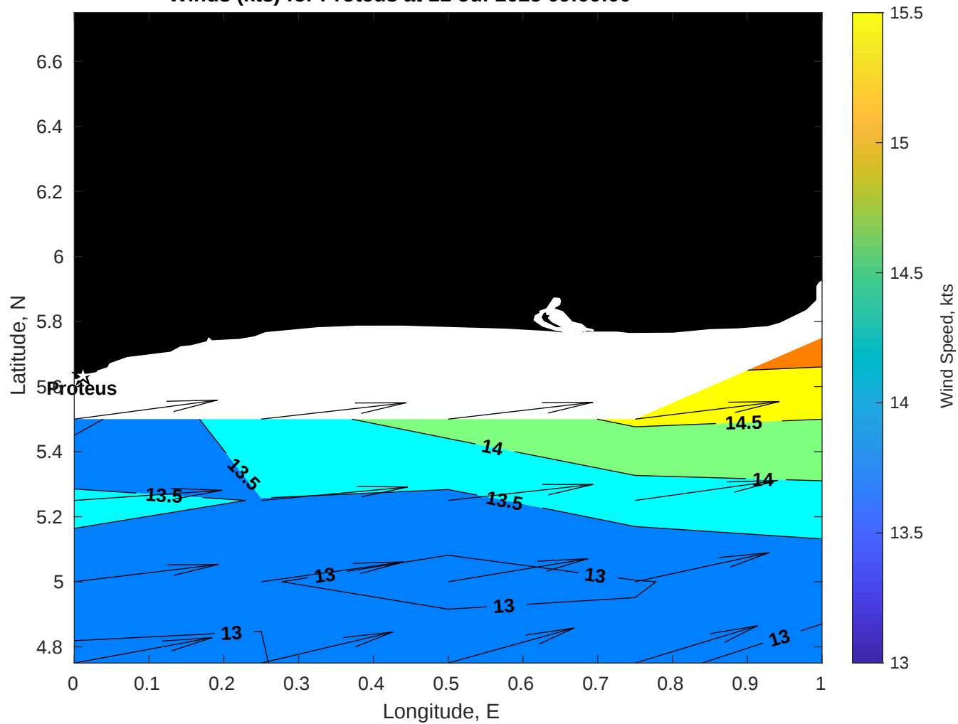
Winds (kts) for Proteus at 11-Jul-2025 09:00:00
