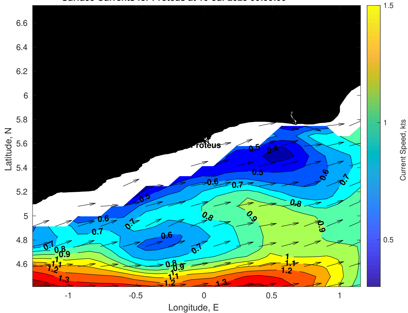
Surface Currents for Proteus at 10-Jul-2025 00:00:00
