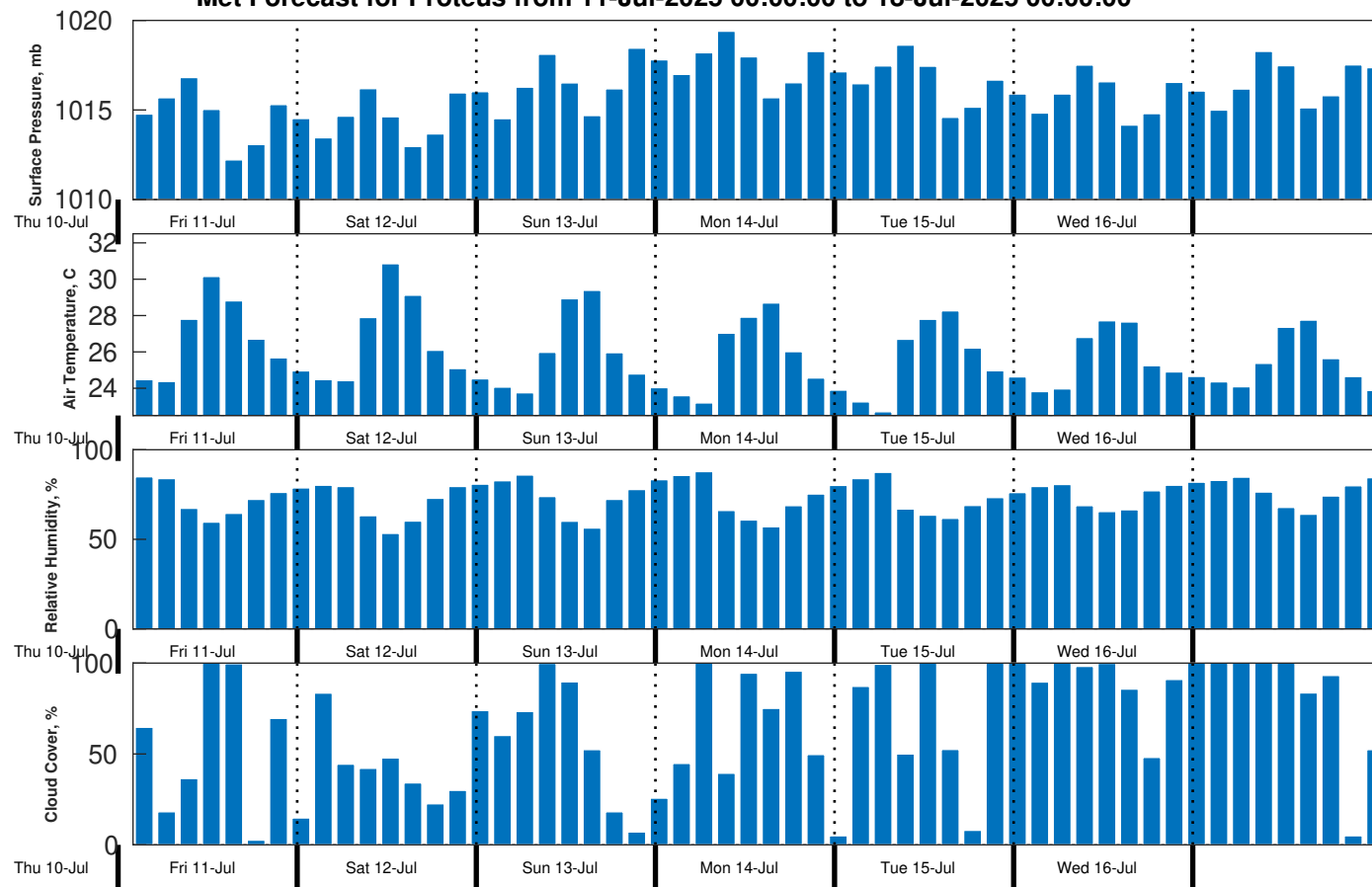
Met Forecast for Proteus from 11-Jul-2025 00:00:00 to 18-Jul-2025 00:00:00
