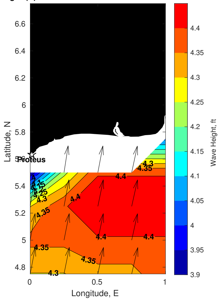
Wave Height (ft) for Proteus at 11-Jul-2025 09:00:00
