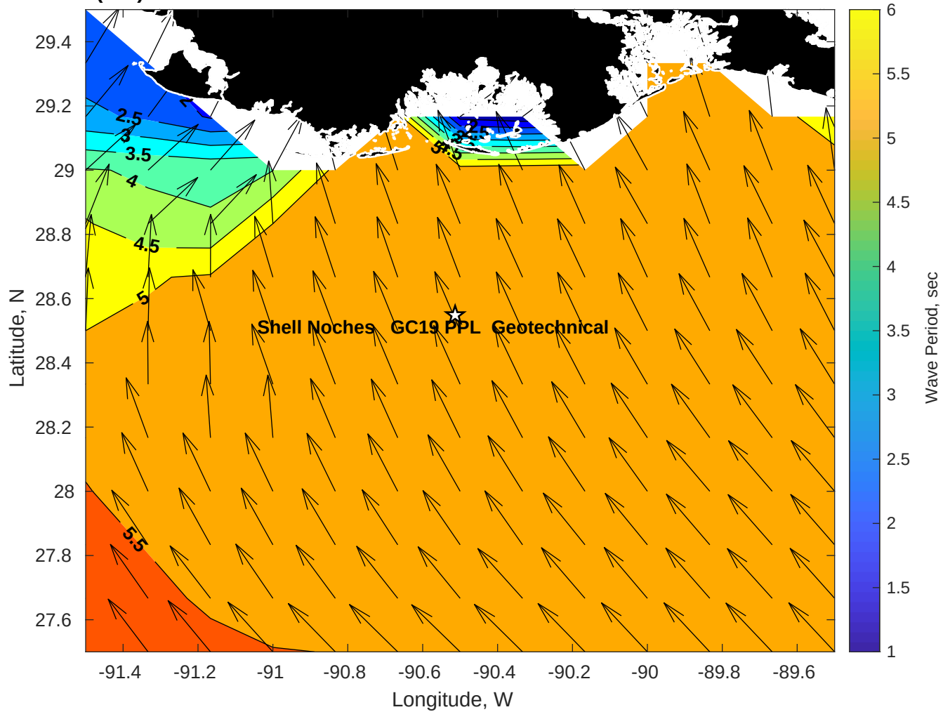
Wave Period (sec) for Shell Noches GC19 PPL Geotechnical at 11-Jul-2025 09:00:00
