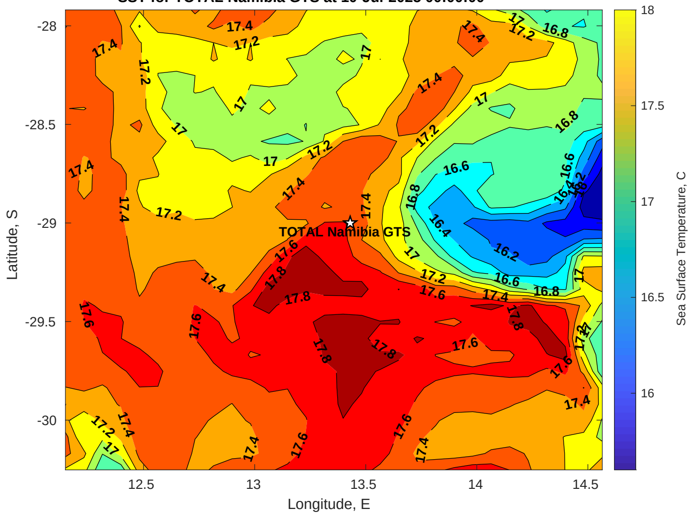
SST for TOTAL Namibia GTS at 10-Jul-2025 00:00:00
