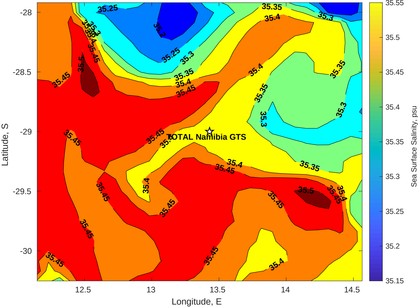
Surface Salinity for TOTAL Namibia GTS at 10-Jul-2025 00:00:00
