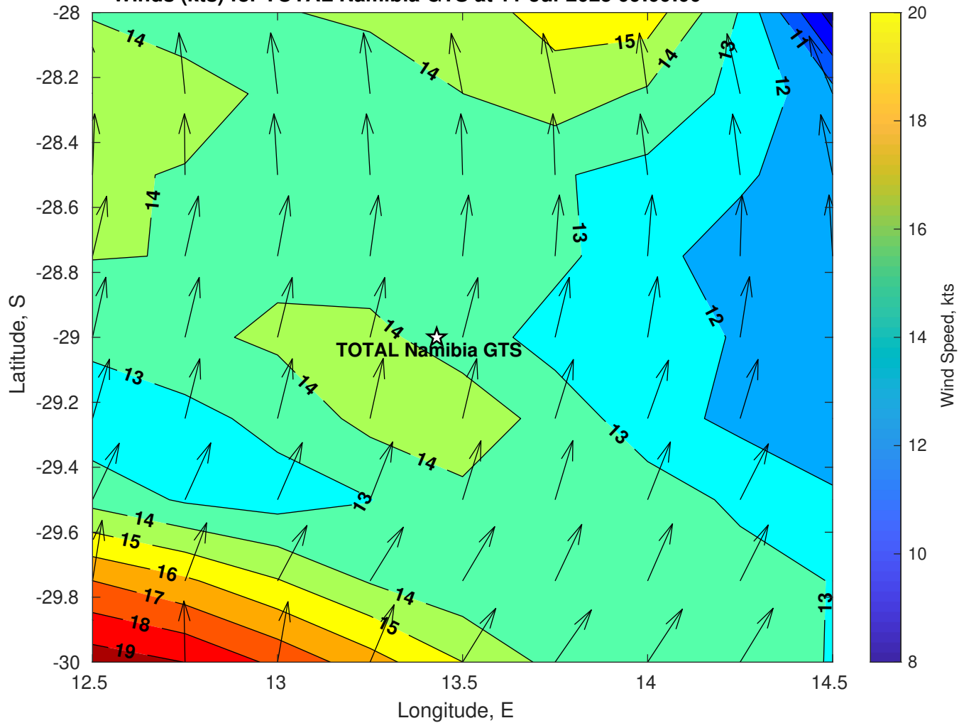
Winds (kts) for TOTAL Namibia GTS at 11-Jul-2025 09:00:00
