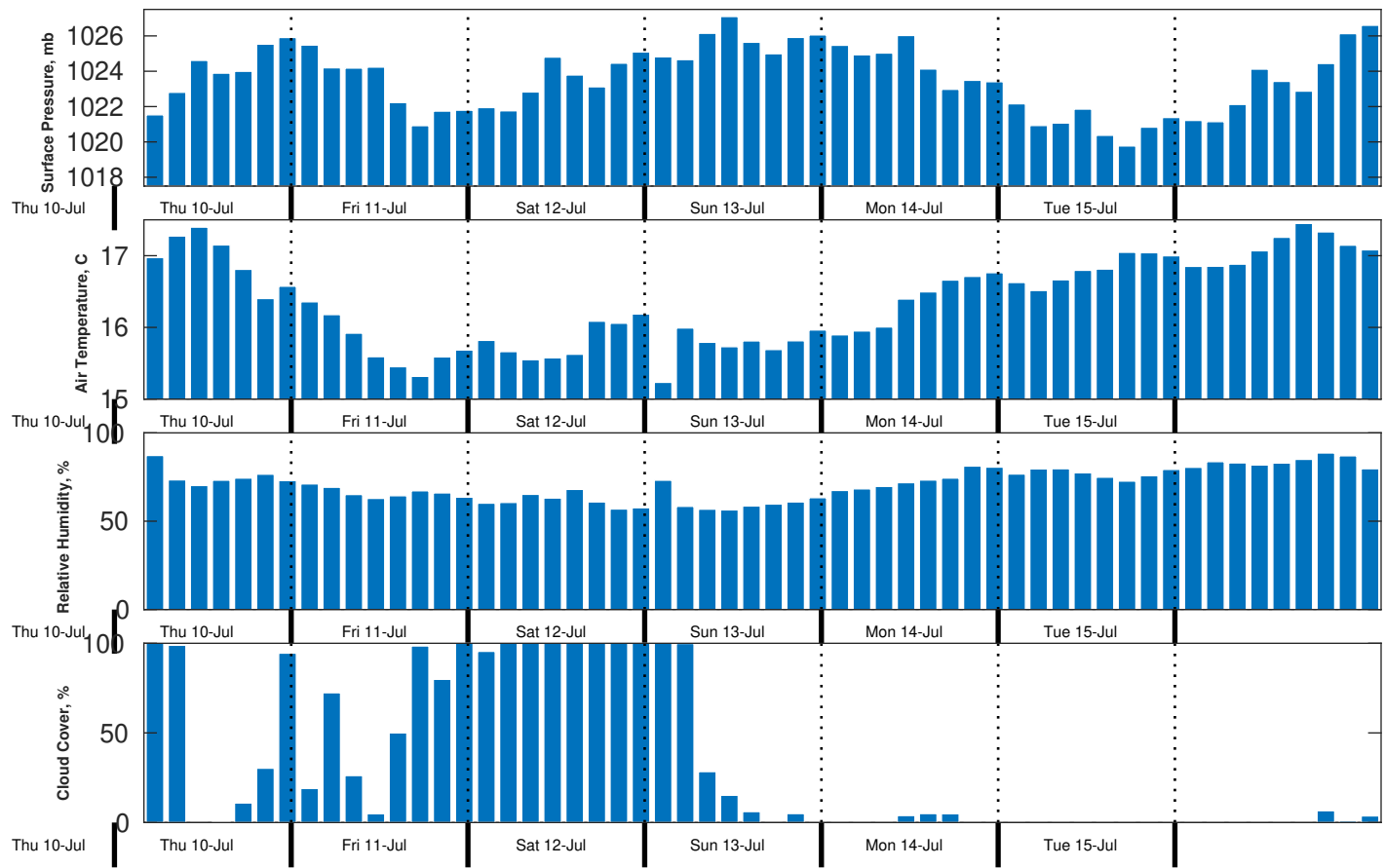
Met Forecast for TOTAL Namibia GTS from 11-Jul-2025 00:00:00 to 18-Jul-2025 00:00:00
