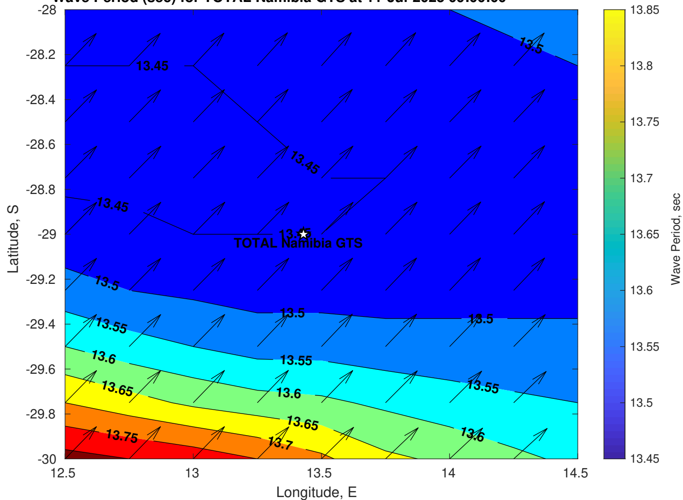
Wave Period (sec) for TOTAL Namibia GTS at 11-Jul-2025 09:00:00
