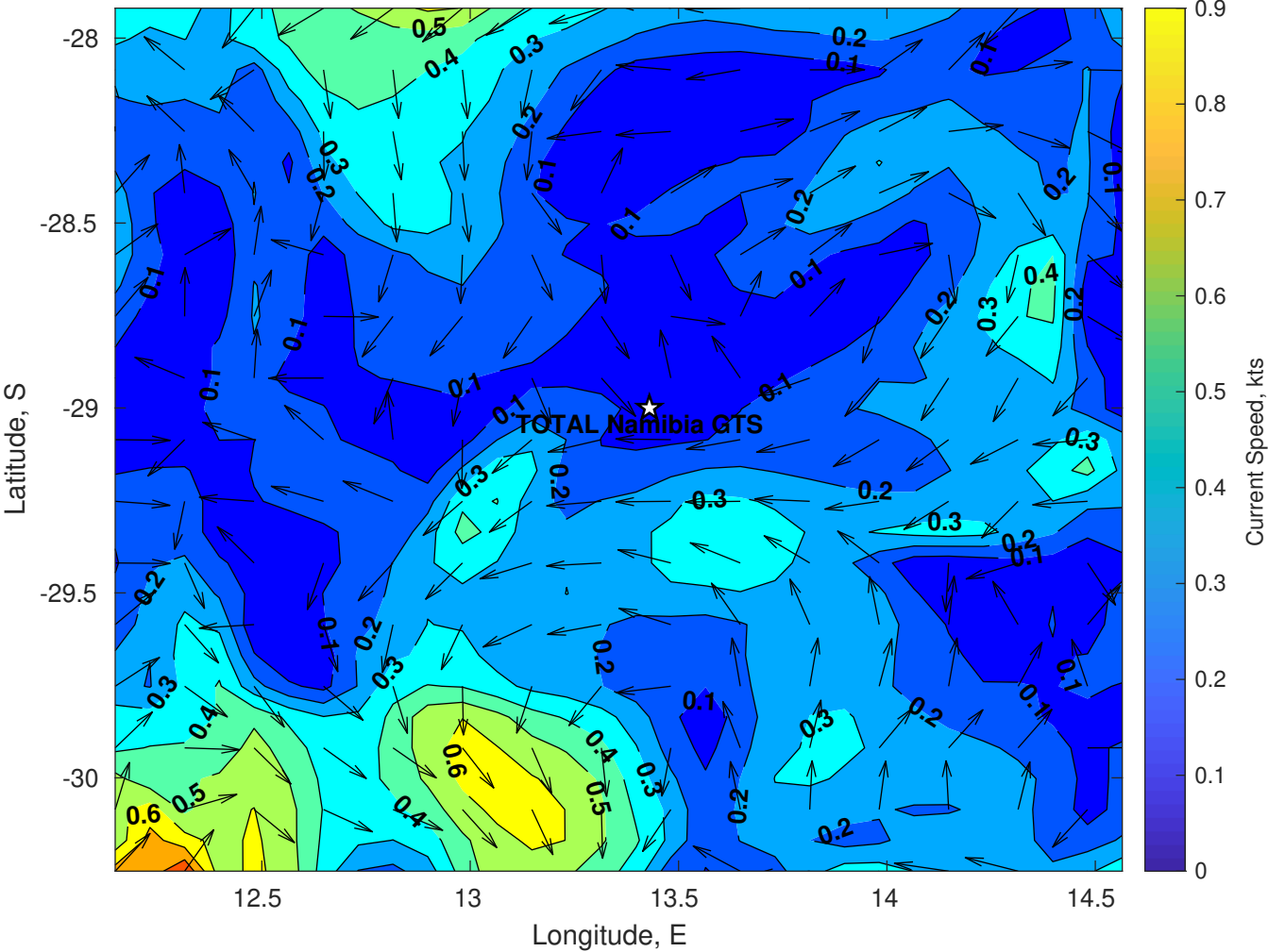
Surface Currents for TOTAL Namibia GTS at 10-Jul-2025 00:00:00
