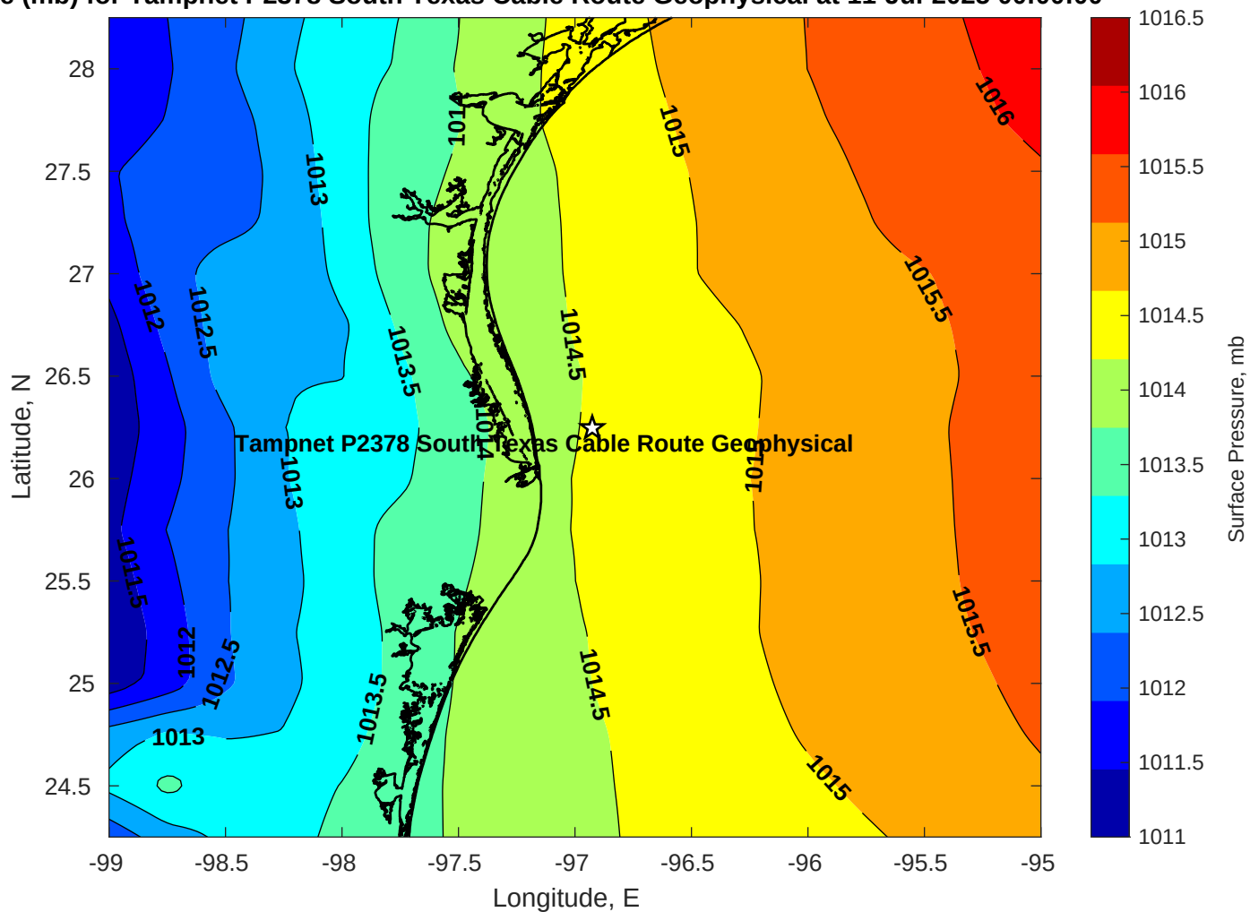
Pressure (mb) for Tampnet P2378 South Texas Cable Route Geophysical at 11-Jul-2025 00:00:00
