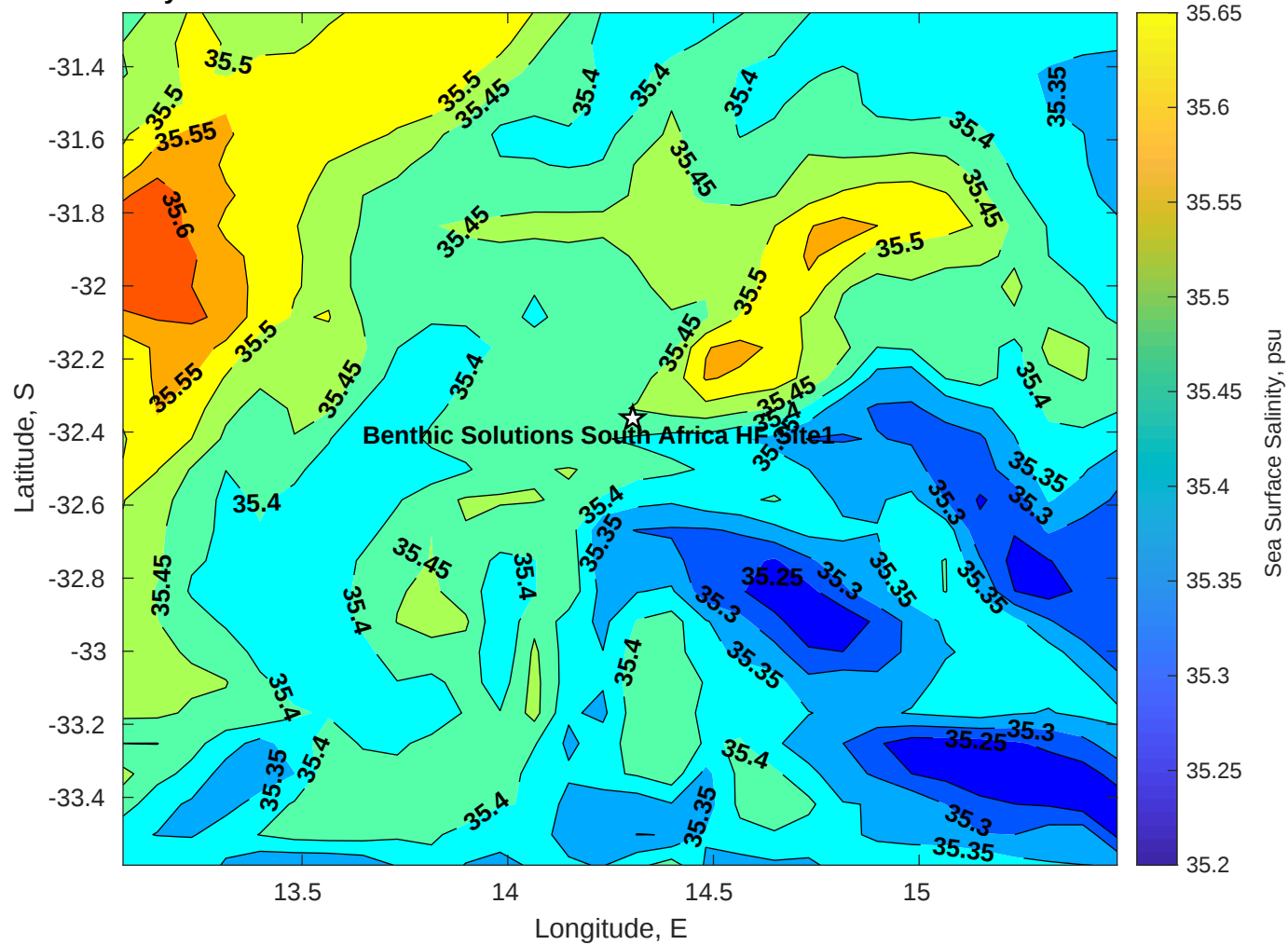
Surface Salinity for Benthic Solutions South Africa HF Site1 at 11-Jul-2025 00:00:00
