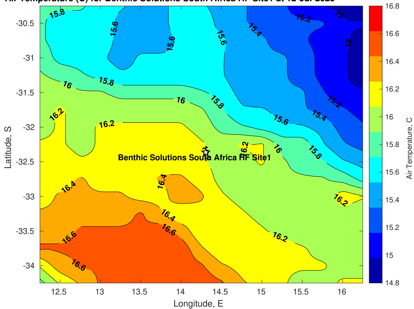
Air Temperature (C) for Benthic Solutions South Africa HF Site1 at 12-Jul-2025
