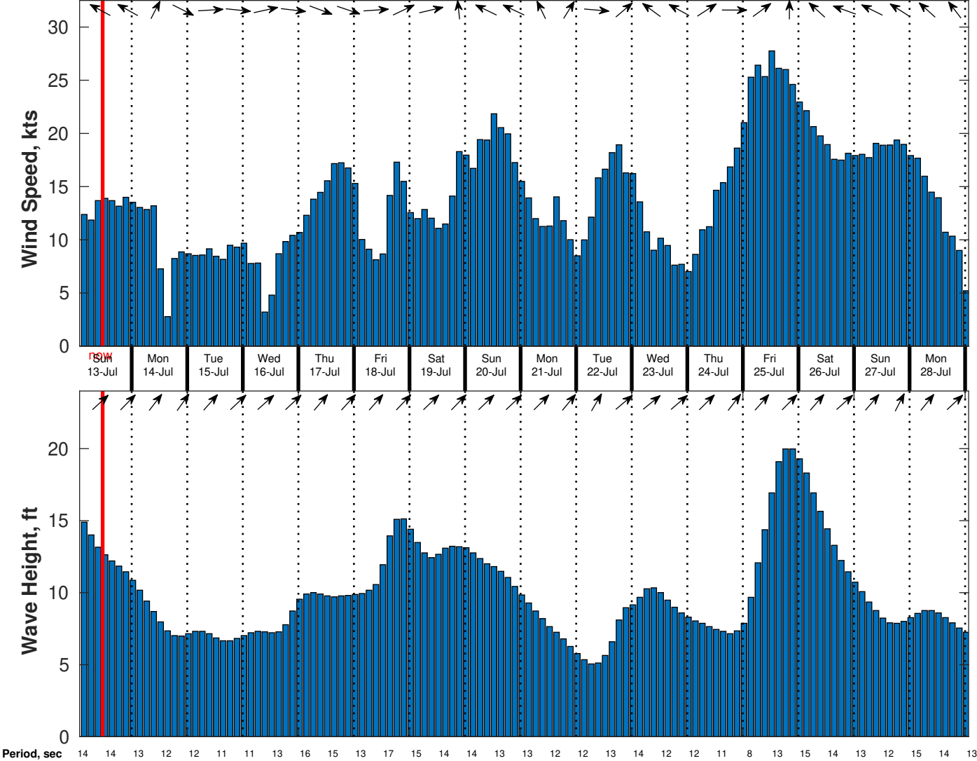
Wind & Wave Forecast for Benthic Solutions South Africa HF Site1 from 12-Jul-2025 02:00:00 to 28-Jul-2025 02:00:00
