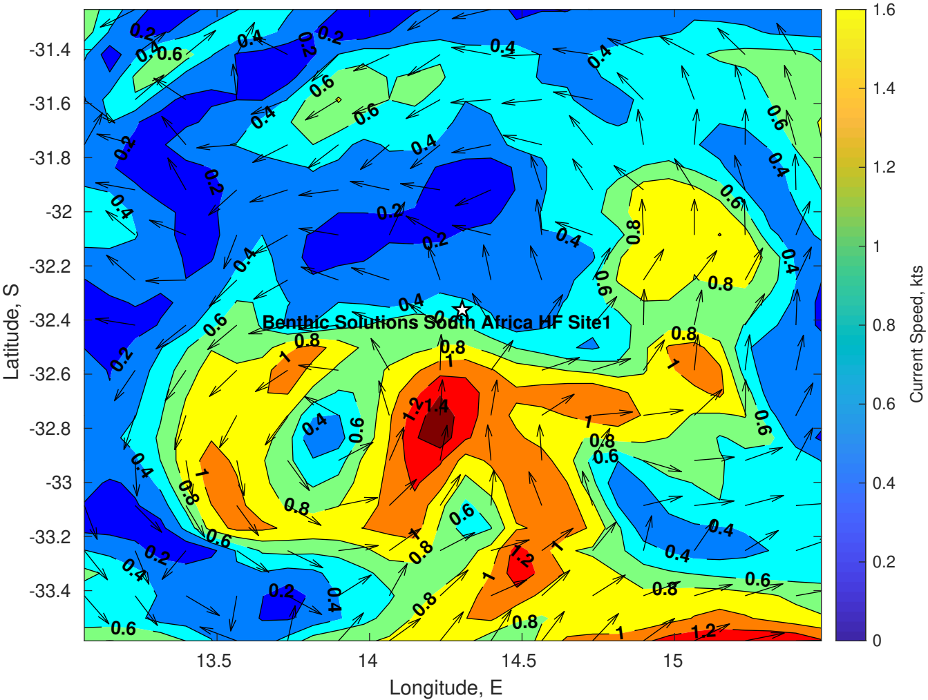
Surface Currents for Benthic Solutions South Africa HF Site1 at 11-Jul-2025 00:00:00
