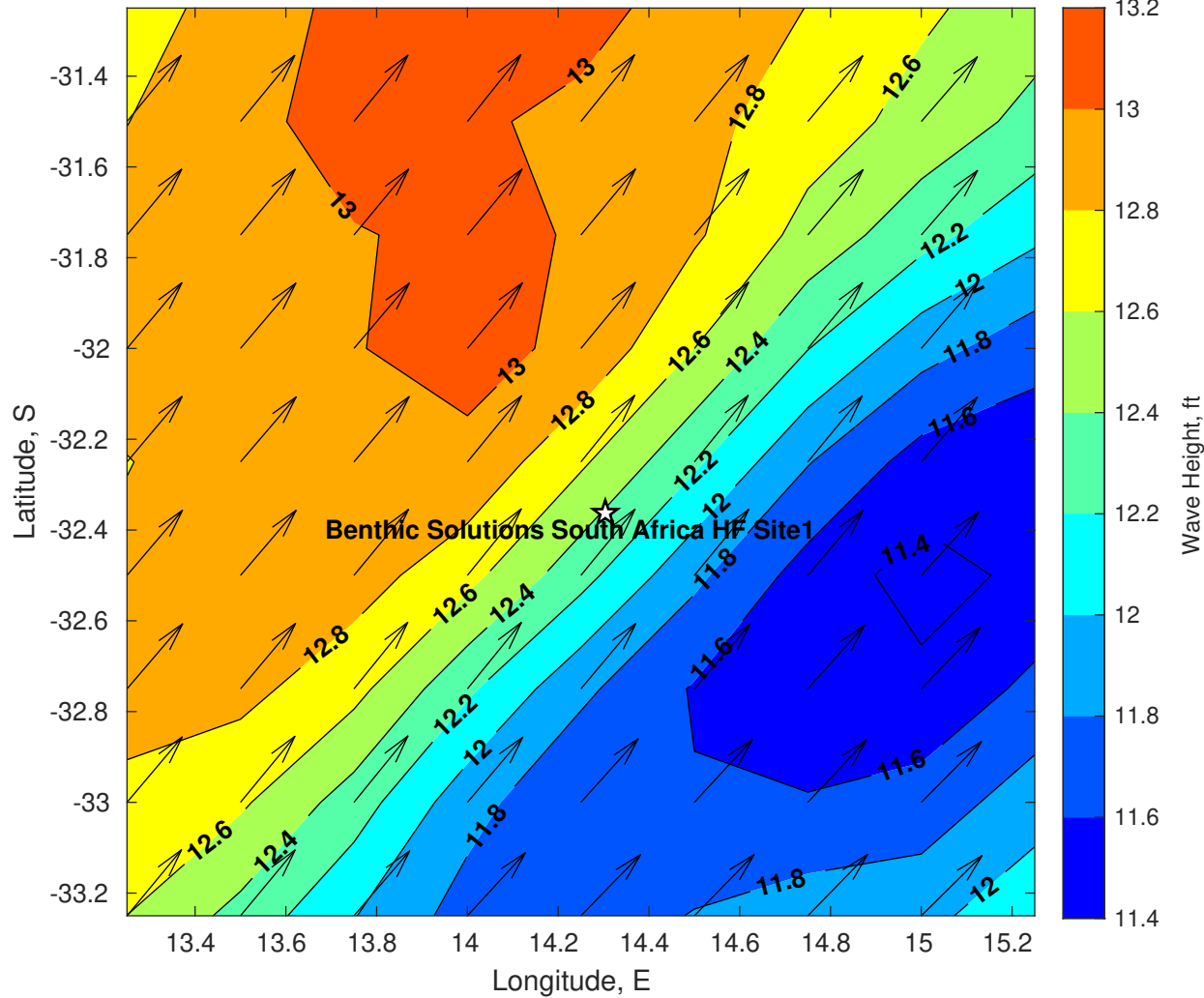
Wave Height (ft) for Benthic Solutions South Africa HF Site1 at 12-Jul-2025 09:00:00
