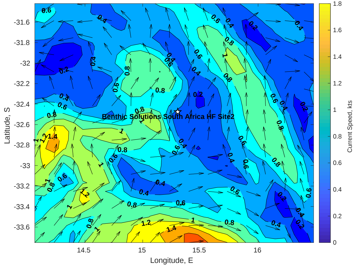
Surface Currents for Benthic Solutions South Africa HF Site2 at 11-Jul-2025 00:00:00
