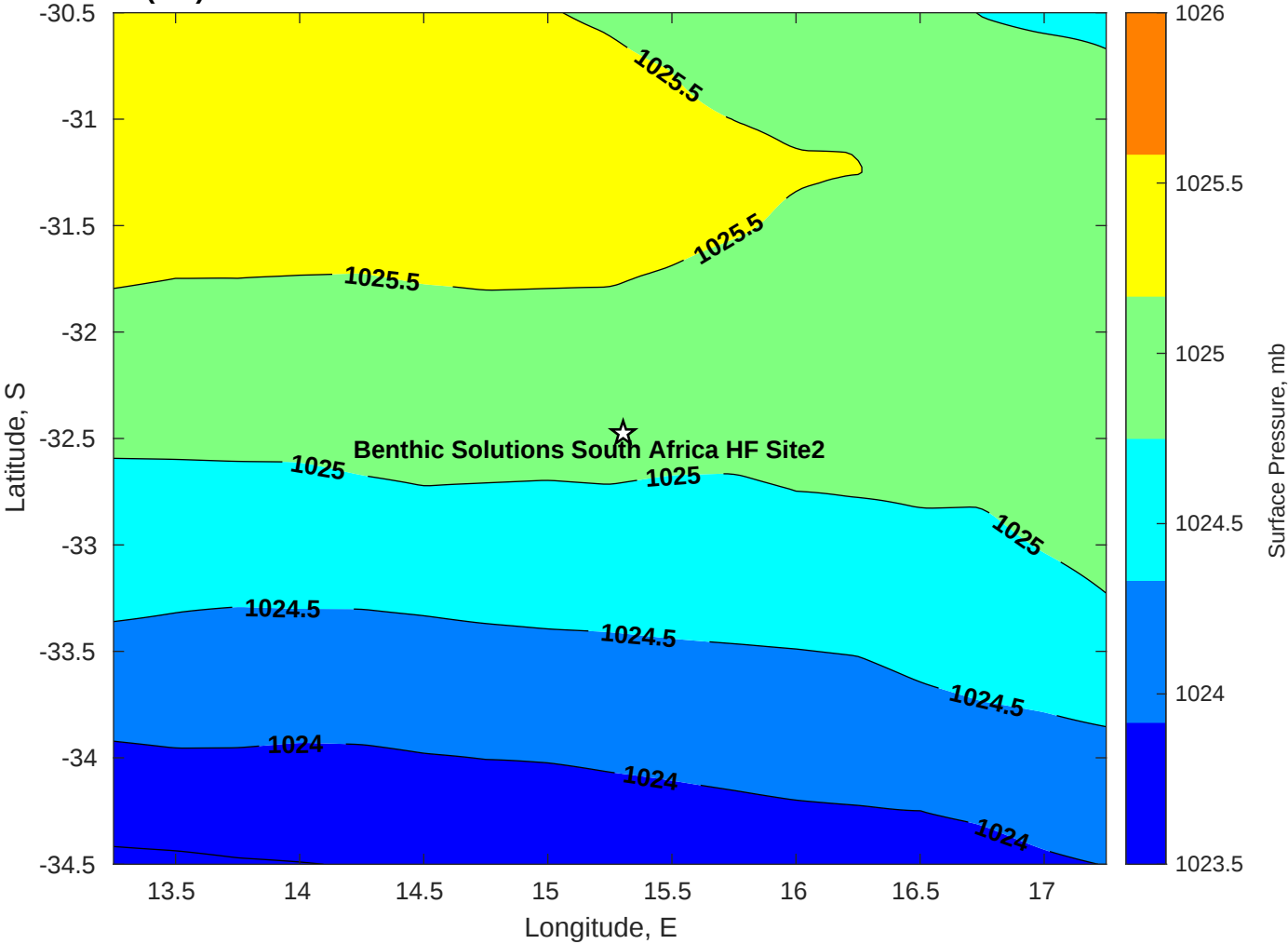
Surface Pressure (mb) for Benthic Solutions South Africa HF Site2 at 14-Jul-2025 00:00:00
