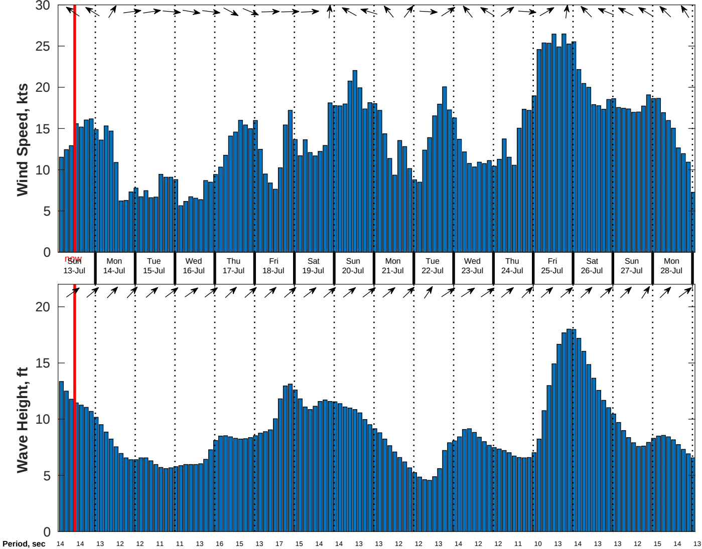
Wind & Wave Forecast for Benthic Solutions South Africa HF Site2 from 12-Jul-2025 02:00:00 to 28-Jul-2025 02:00:00
