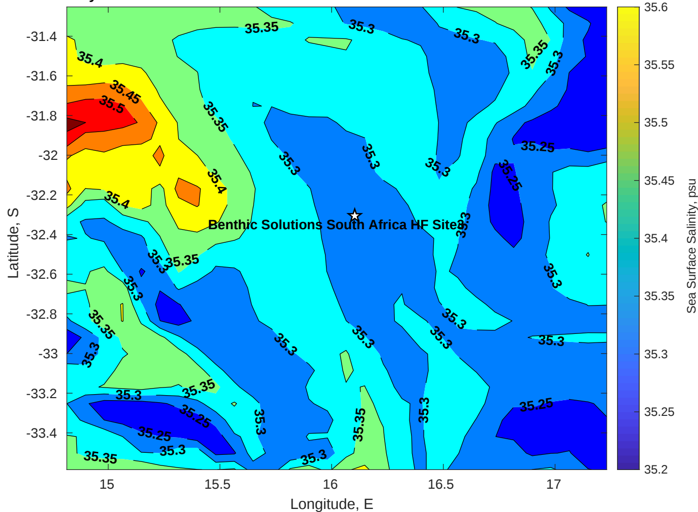
Surface Salinity for Benthic Solutions South Africa HF Site3 at 11-Jul-2025 00:00:00
