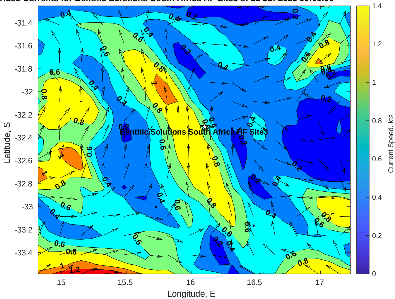
Surface Currents for Benthic Solutions South Africa HF Site3 at 11-Jul-2025 00:00:00
