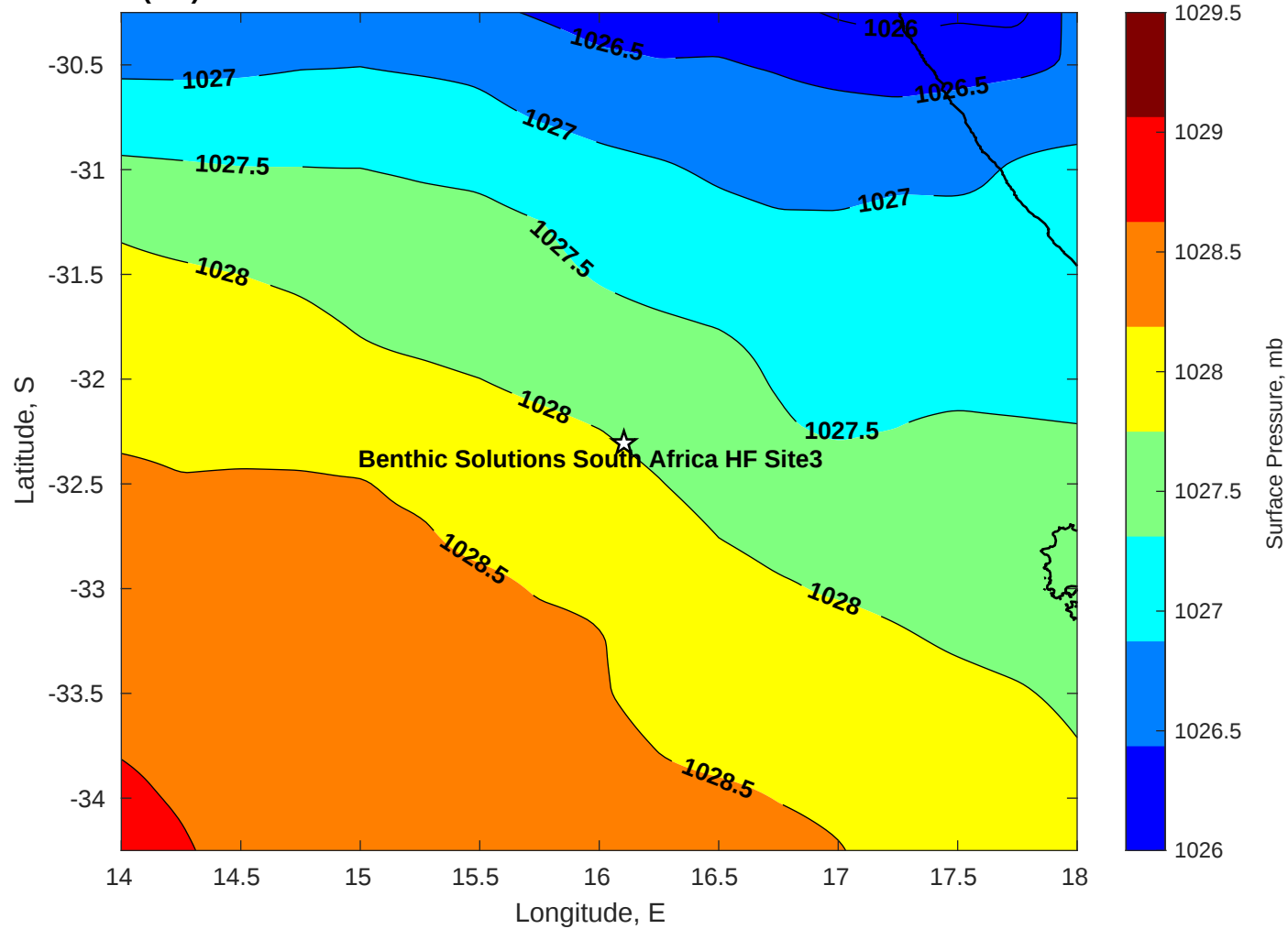
Surface Pressure (mb) for Benthic Solutions South Africa HF Site3 at 12-Jul-2025 00:00:00
