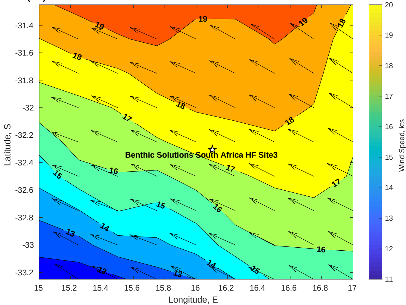
Winds (kts) for Benthic Solutions South Africa HF Site3 at 12-Jul-2025 09:00:00
