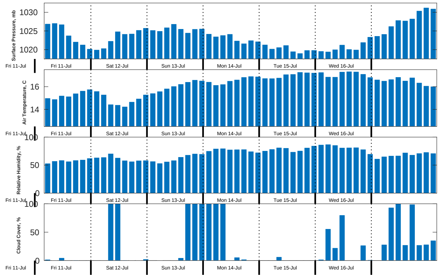
Met Forecast for Benthic Solutions South Africa HF Site3 from 12-Jul-2025 00:00:00 to 19-Jul-2025 00:00:00
