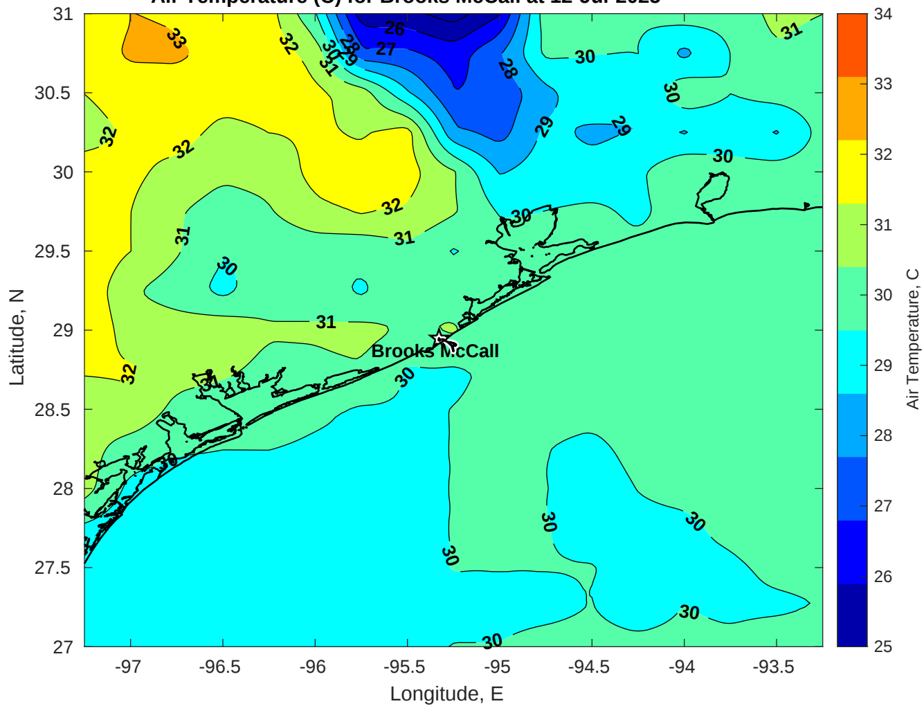
Air Temperature (C) for Brooks McCall at 12-Jul-2025
