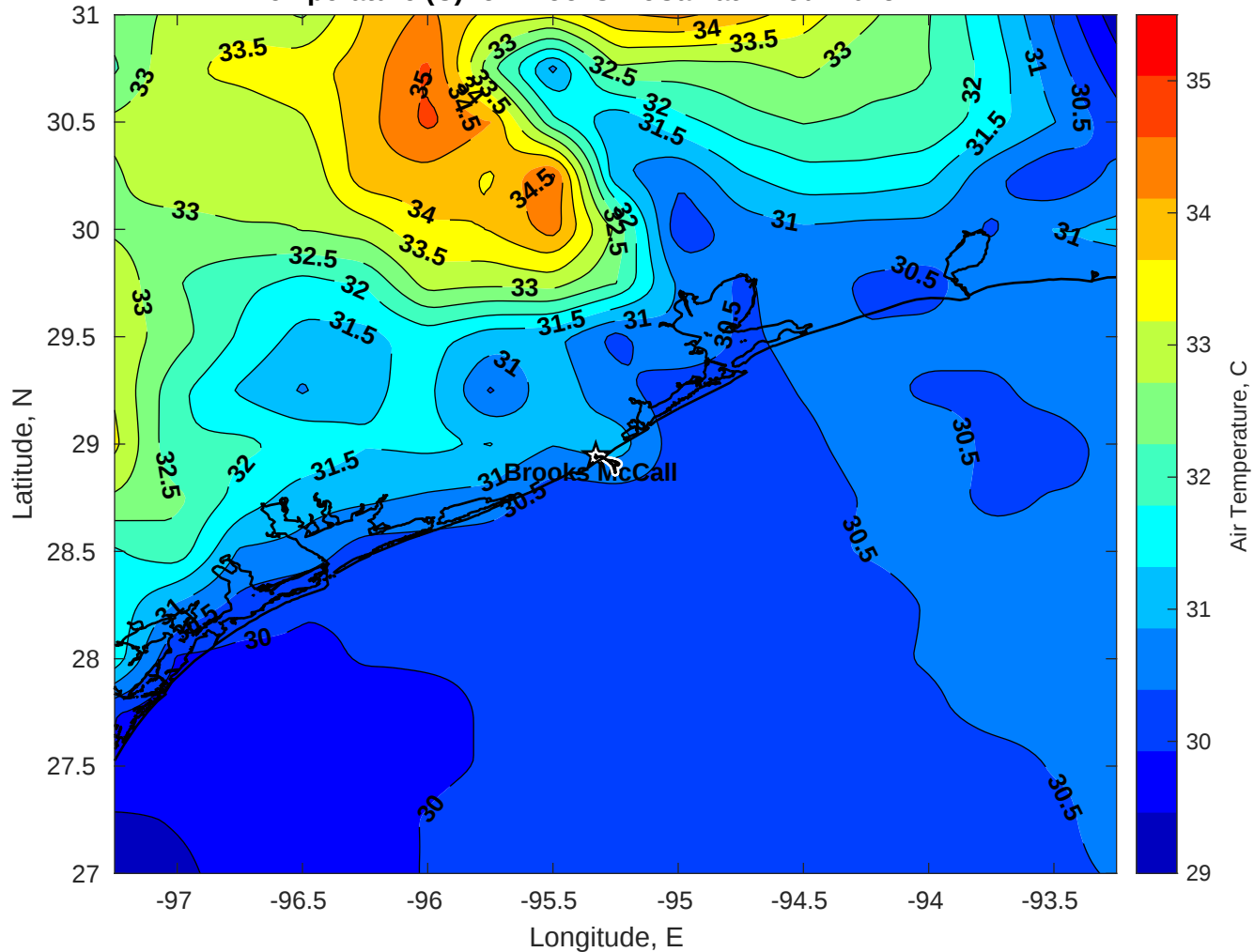
Air Temperature (C) for Brooks McCall at 12-Jul-2025
