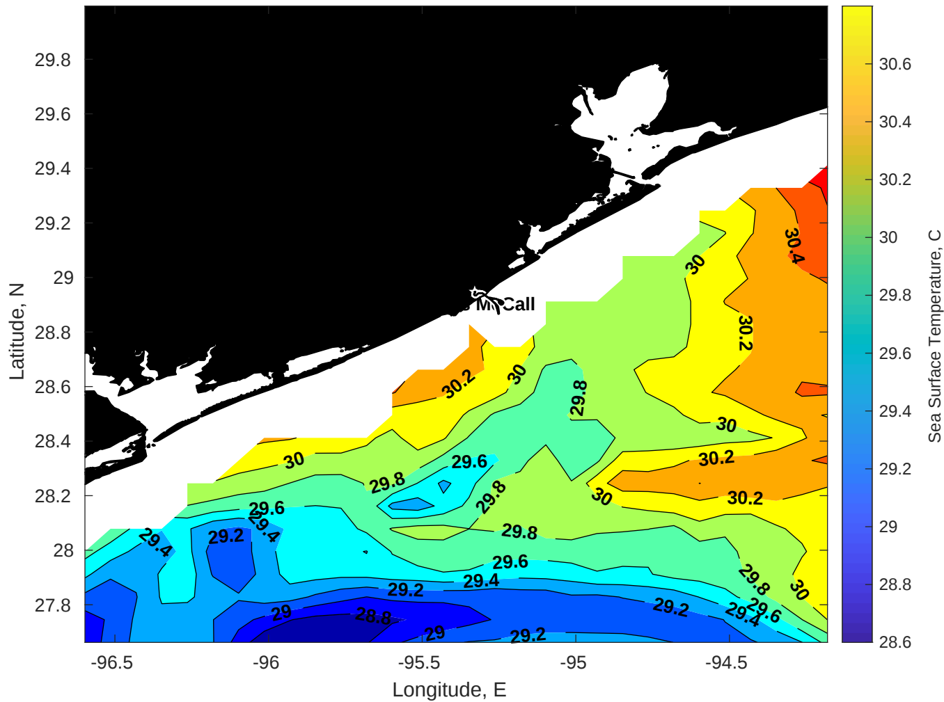
SST for Brooks McCall at 11-Jul-2025 00:00:00
