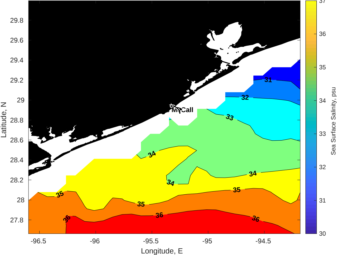
Surface Salinity for Brooks McCall at 11-Jul-2025 00:00:00
