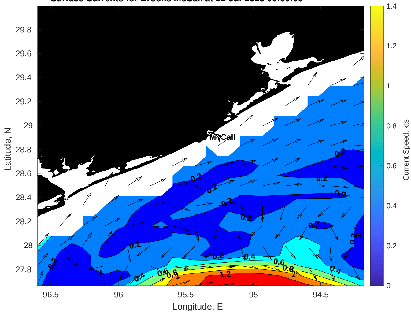
Surface Currents for Brooks McCall at 11-Jul-2025 00:00:00
