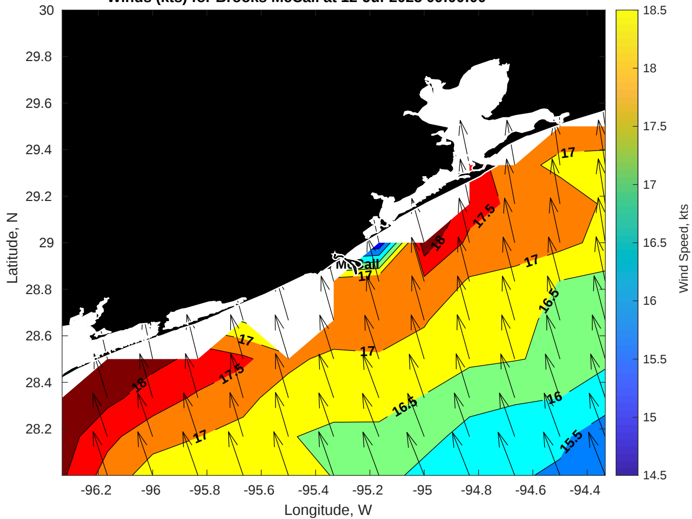
Winds (kts) for Brooks McCall at 12-Jul-2025 09:00:00
