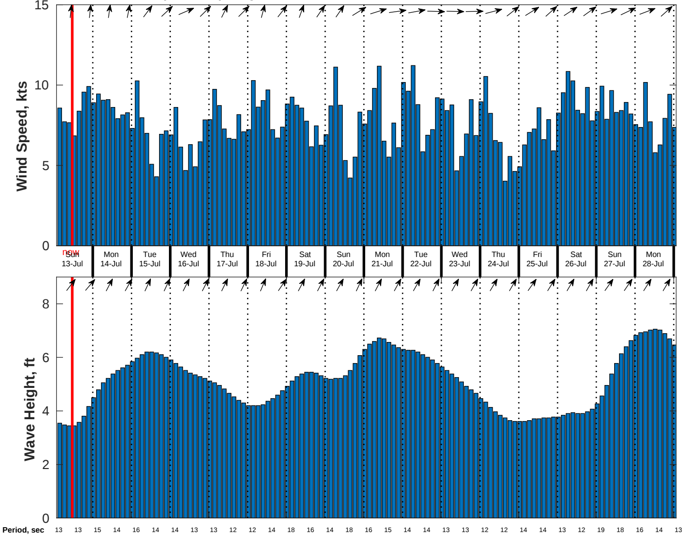
Wind & Wave Forecast for CABGOC (Chevron) Angola BLK 14 EBS from 12-Jul-2025 02:00:00 to 28-Jul-2025 02:00:00
