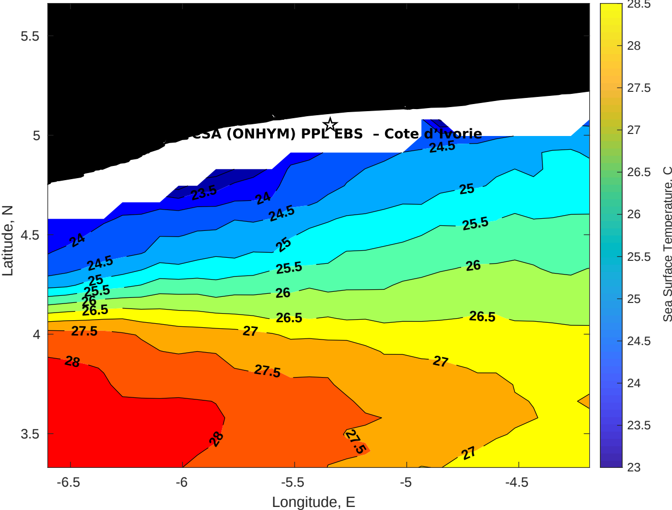
SST for CSA (ONHYM) PPL EBS - Cote d'Ivoire at 11-Jul-2025 00:00:00
