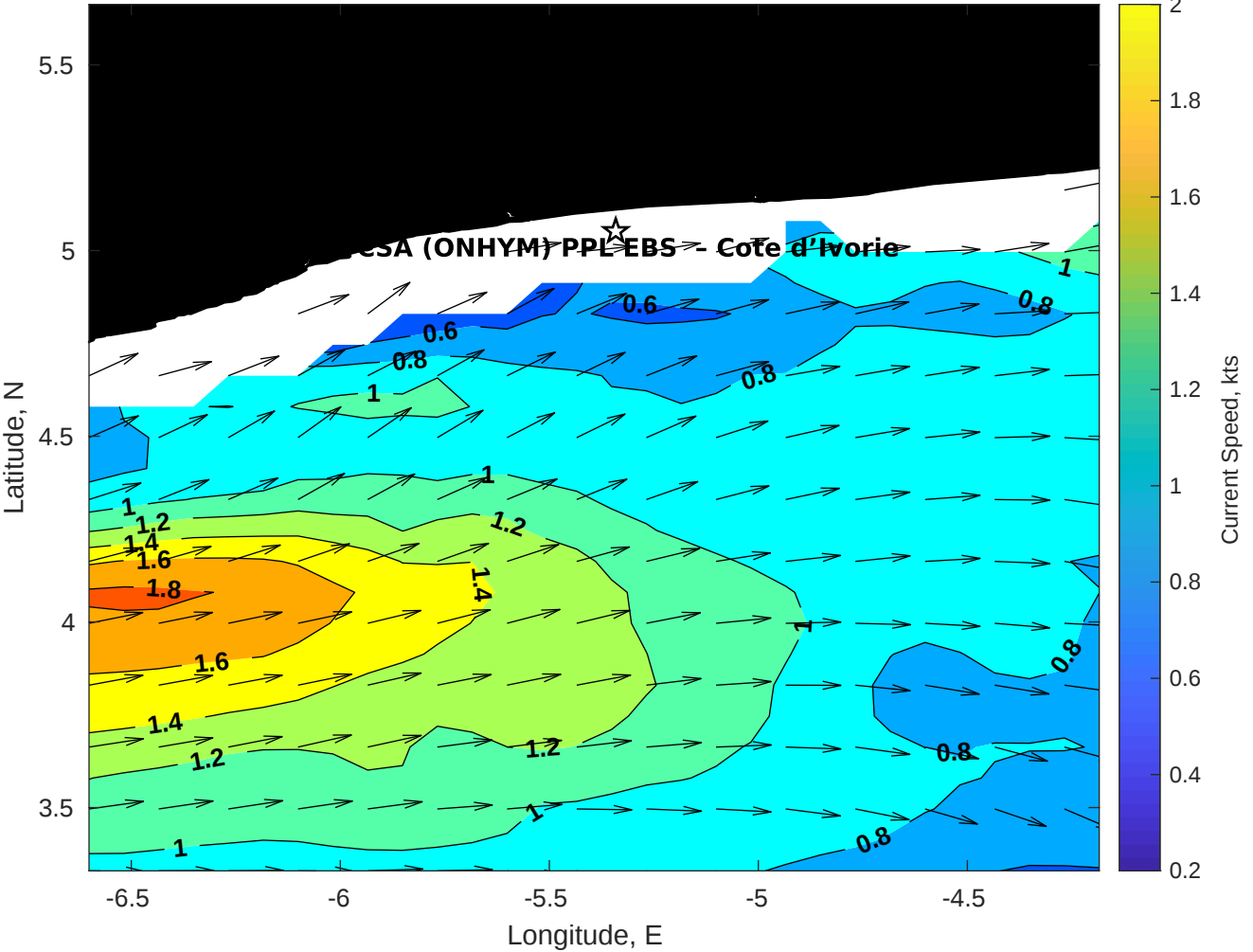
Surface Currents for CSA (ONHYM) PPL EBS - Cote d'Ivoire at 11-Jul-2025 00:00:00
